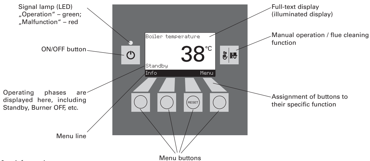
Fig. 10 Info panel
