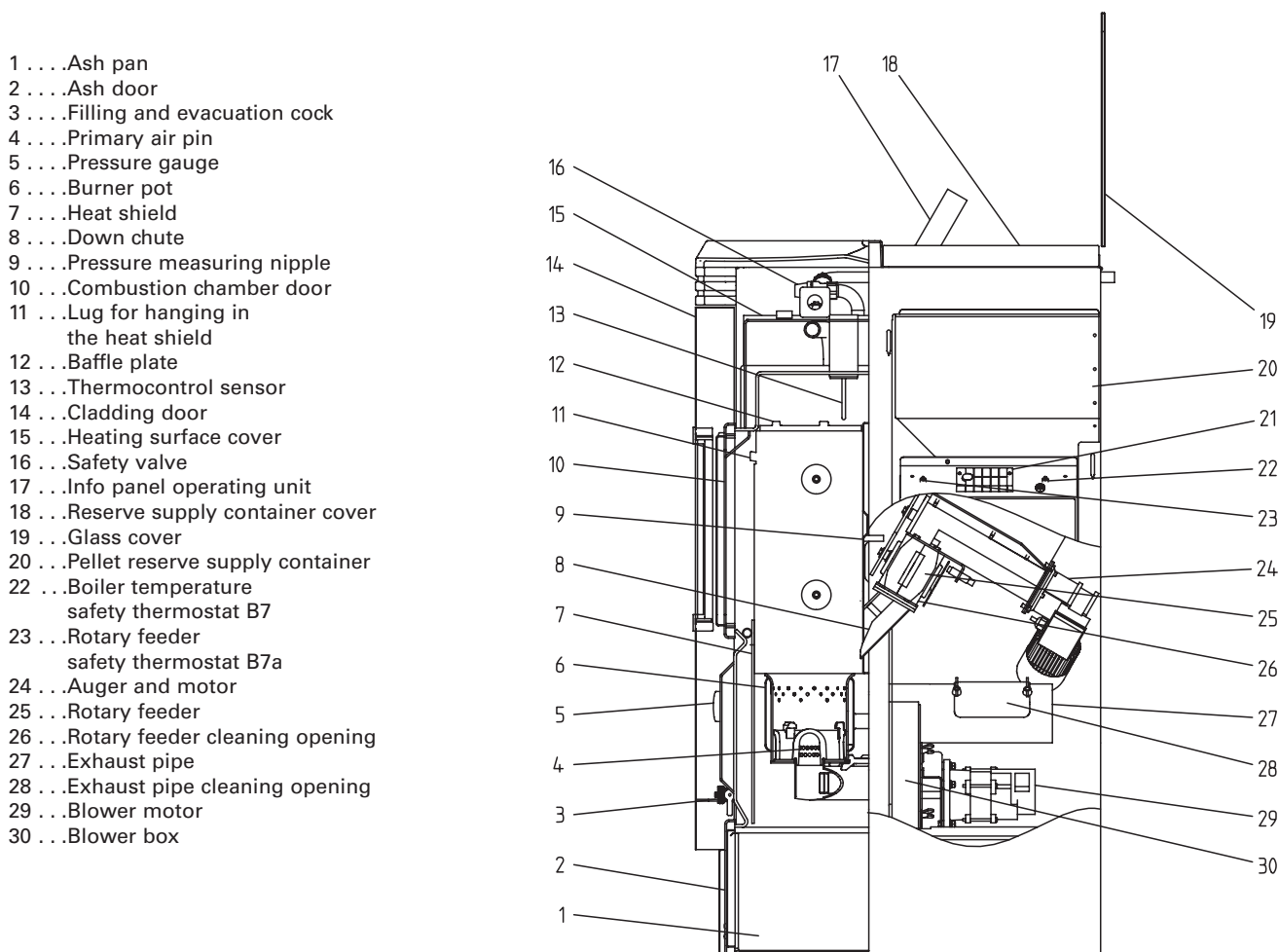
Fig. 3 BAXI Bioflo – view from right
