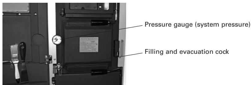
Fig. 6 Filling the system
