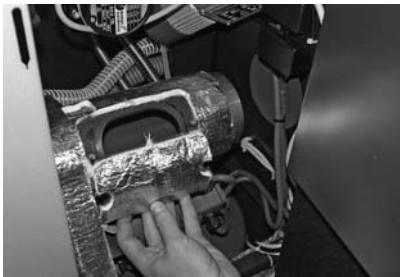
Fig. 99 Removing the wing nuts and cleaning opening – cleaning the exhaust pipe
