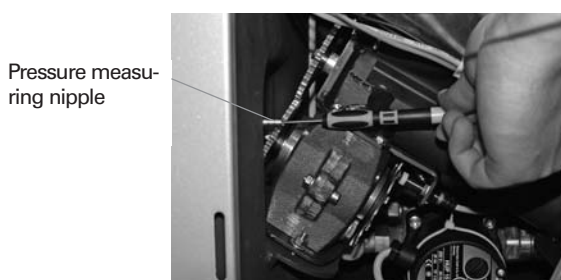
Fig. 97 Cleaning the induction opening with a small screwdriver or the like
