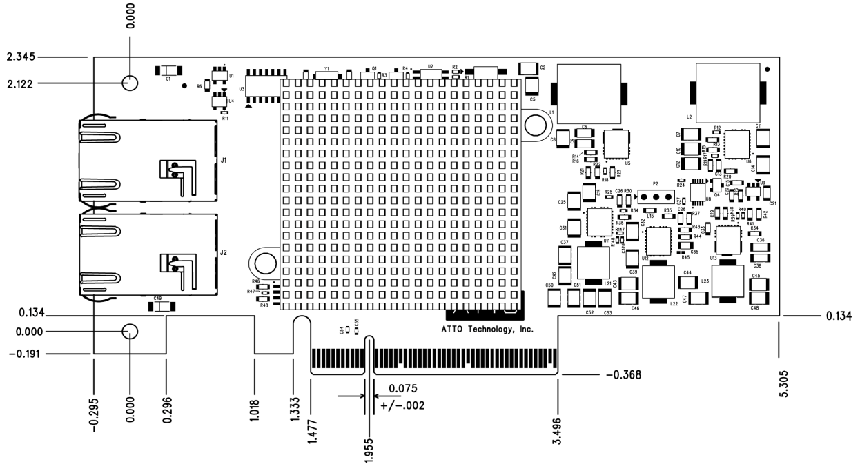
Exhibit 3-9 FFRM-NT12 board
