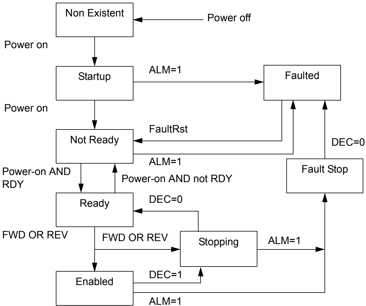
Figure 12. ODVA state transition diagram Speed Actual (AC/DC Drive Object)
