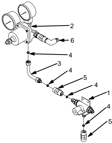
FIGURE 31. REGULATOR ASS'Y, HI-PRESSURE (P/N 0650)
