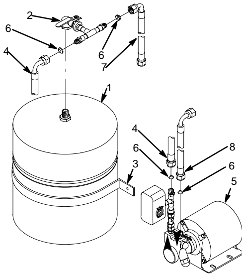
FIGURE 26. WATER OUTLET VALVE ASS'Y (P/N 0193)
