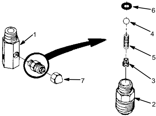
FIGURE 22. CHECK VALVE AND MANIFOLD ASS'Y (P/N 183302-100)
