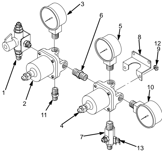
FIGURE 19. CO 2 CHECK VALVE ASS'Y (P/N 183301-001)
