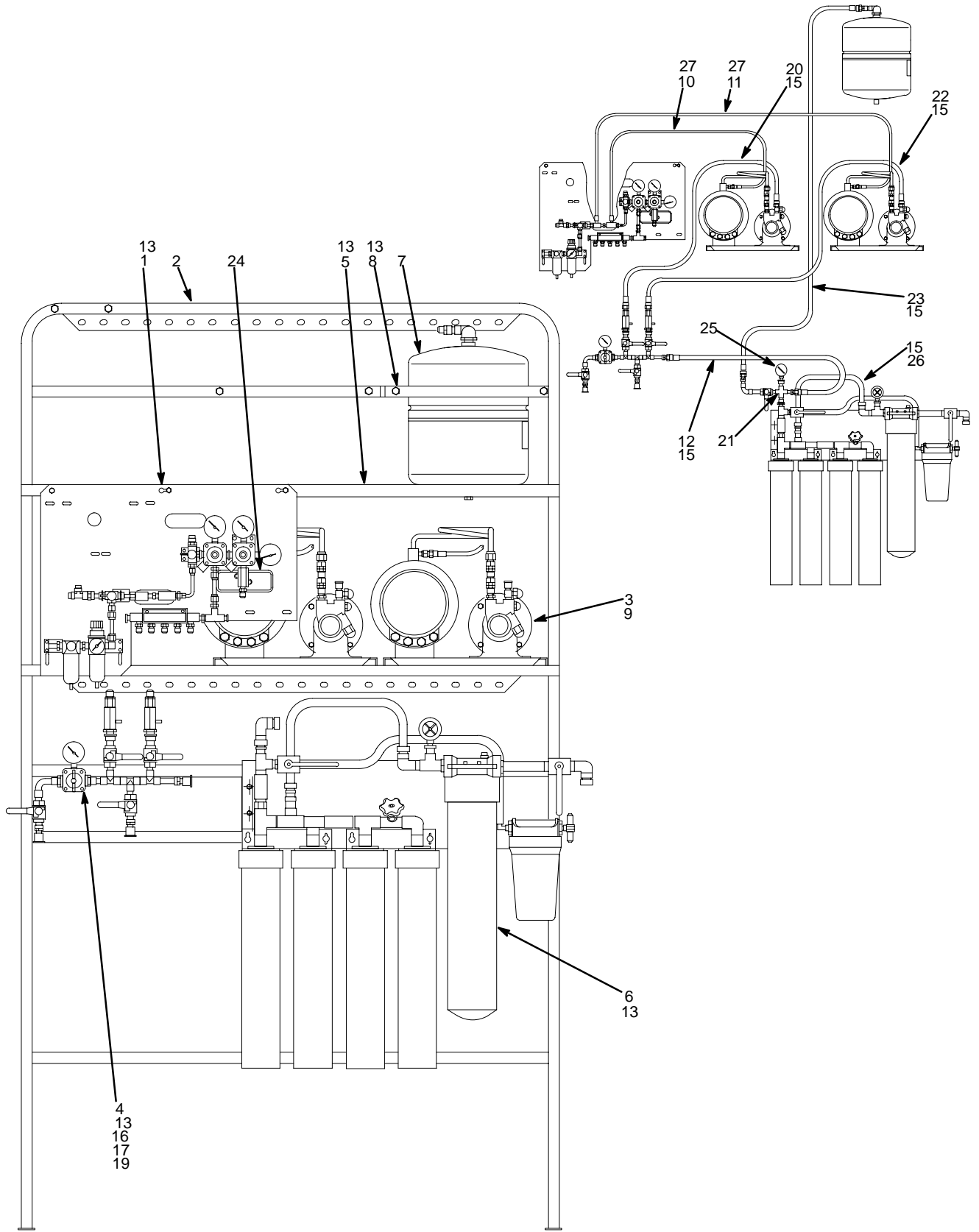
FIGURE 16. BEVERAGE CONTROL PANEL ASS'Y
