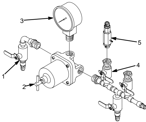
FIGURE 25. WATER MANIFOLD ASS'Y (P/N 300914-000)
