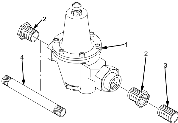
FIGURE 33. OPTIONAL WATER PRESSURE REGULATOR KIT (P/N 300919-000)
