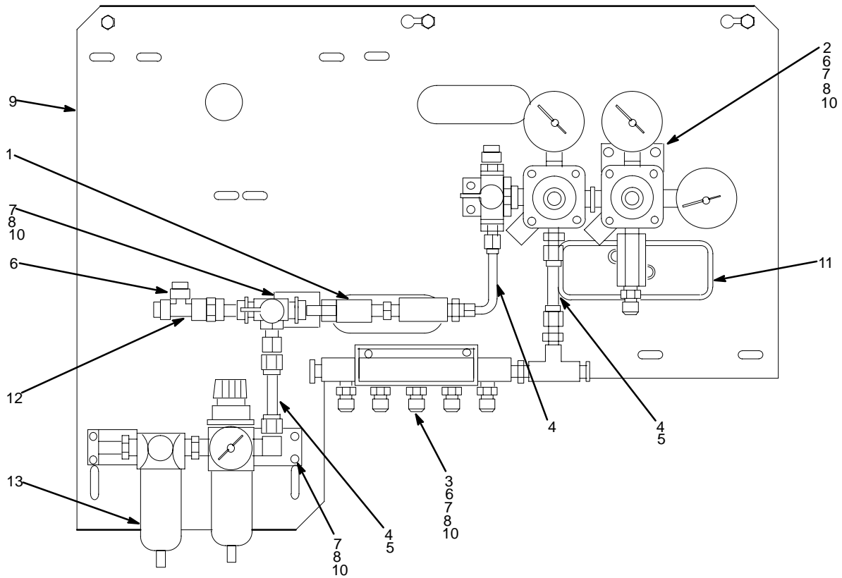
FIGURE 17. CO 2 REGULATOR ASS'Y (P/N 0483)
