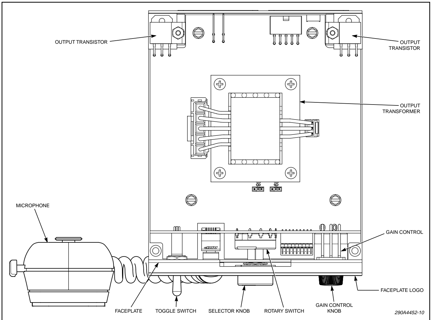
Figure 5-1. Internal View.
