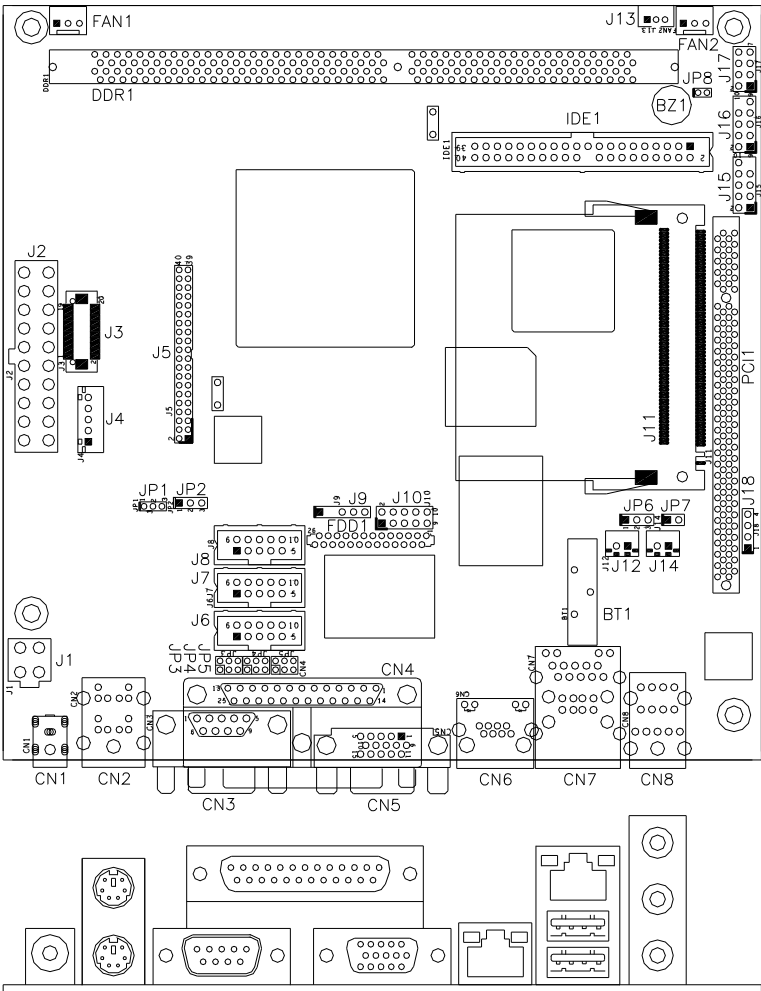
Connectors on MB500
