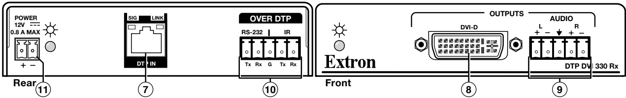
Figure 3. DTP DVI 330 Rx Connectors
