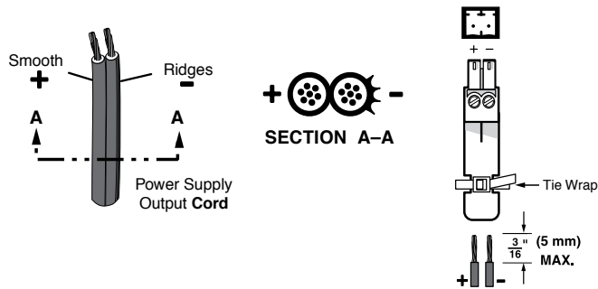
Figure 6. Power Connector Wiring
