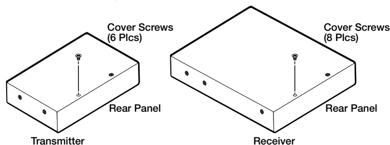
Figure 9. Opening the Transmitter and Receiver
