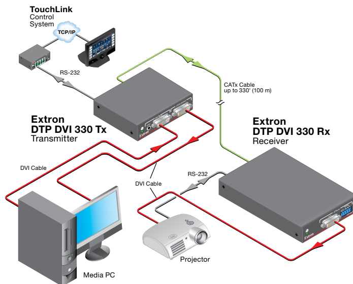
Figure 1. Typical Transmitter and Receiver Application
