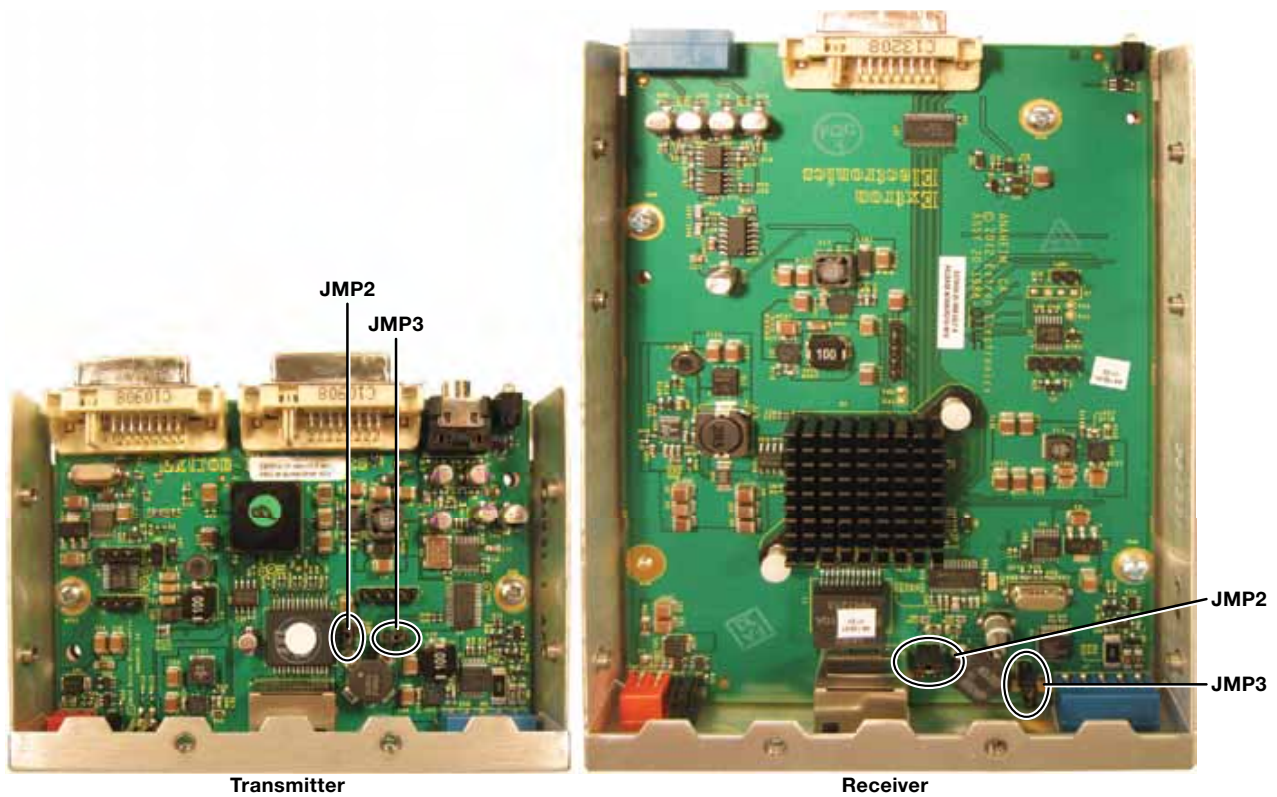
Figure 10. Jumper Locations
