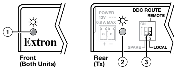
Figure 8. Power Indicators
