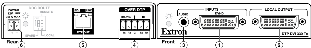
Figure 2. DTP DVI 330 Tx Connectors
