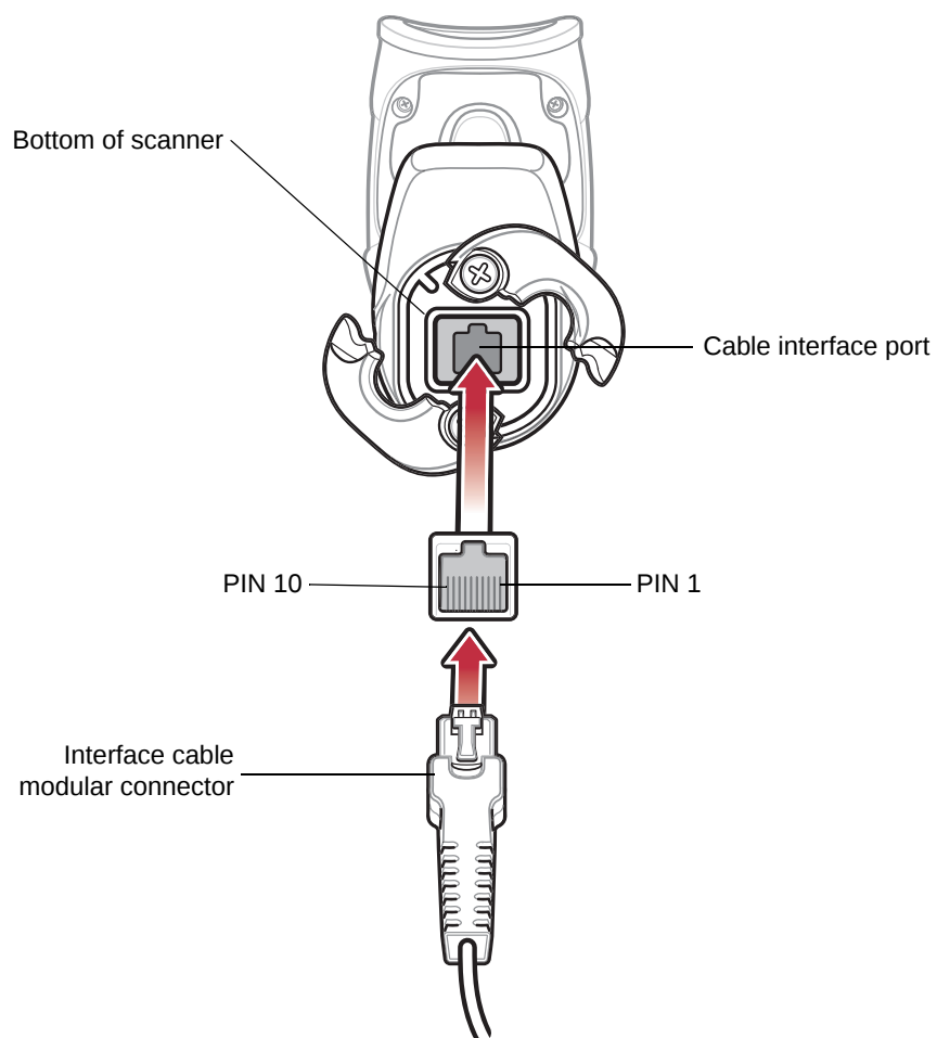
Figure 3-1 Digital Scanner Cable Pinouts
