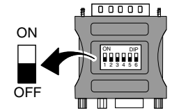
MAC/VGA ADAPTER
