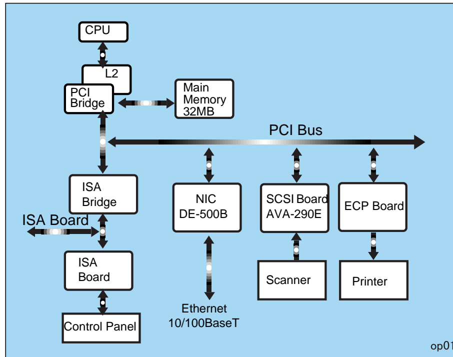
Figure 2-1. System Connection
