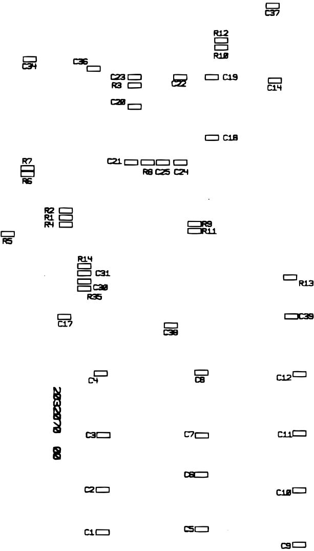
Figure 7-3. C85010 I/F (ISA Board) Component Layout (2)
