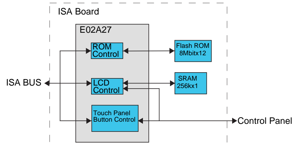
Figure 2-2. ISA Board Block Diagram
