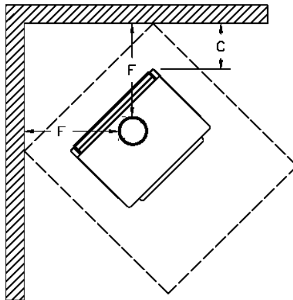
Clearances to combustibles and floor protection
