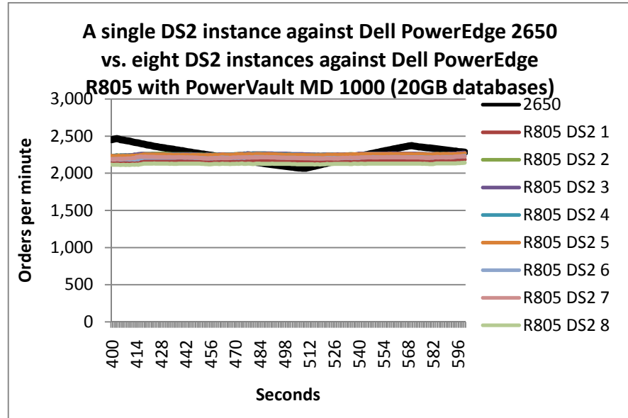
Figure 3. A single DS2 instance running on a Dell PowerEdge 2650 vs. eight DS2 instances running on a Dell PowerEdge R805 and PowerVault MD 1000, during a period of steady activity, using eight DS2 20GB databases. Higher numbers of orders per minute are better.
