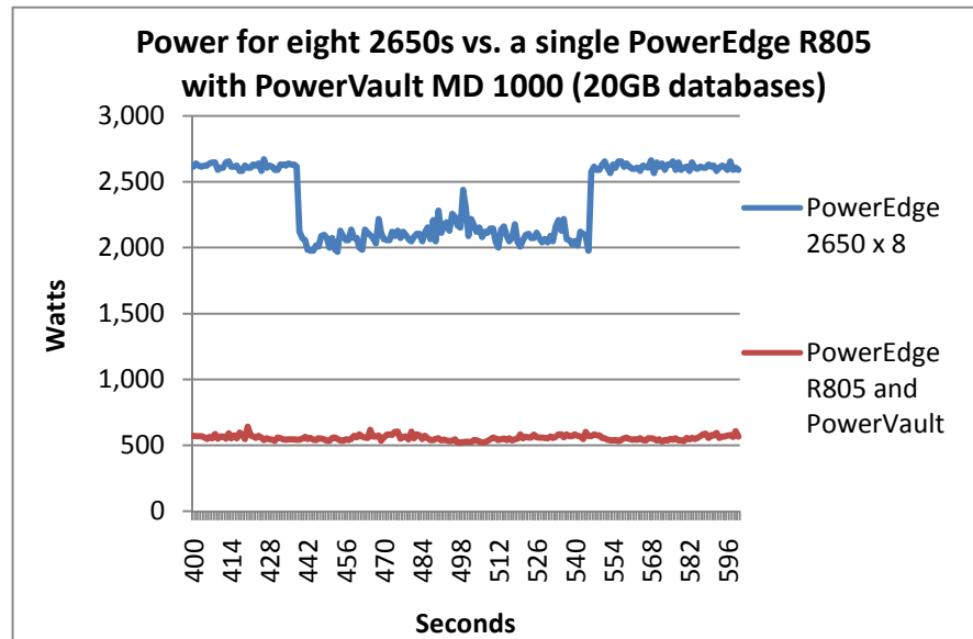
Figure 5. Power usage for eight Dell PowerEdge 2650 servers vs. a single PowerEdge R805 server with PowerVault MD 1000, in Watts, when using eight DS2 20GB databases. Lower power usage is better.
