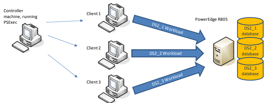
Figure 12. Sample test topology for the Dell PowerEdge R805 with three sample workload-generating systems.
