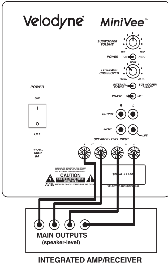
Figure 3. Installation Using Speaker-Level Inputs
