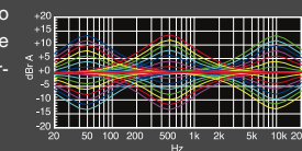
Audio Precision (Bass Midrange Treble)
