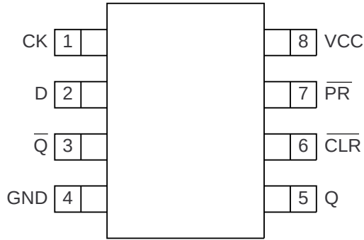
IC1: VHiTC7WT74FU1 (TC7WT74)
