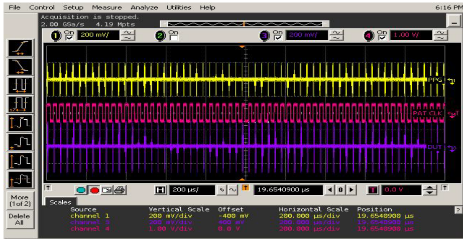
Figure - 4 Example OOB-07 test stimulus and PUT response, for nominal COMINIT/COMRESET gap (Test stimulus top, yellow. PUT response bottom, purple.)
