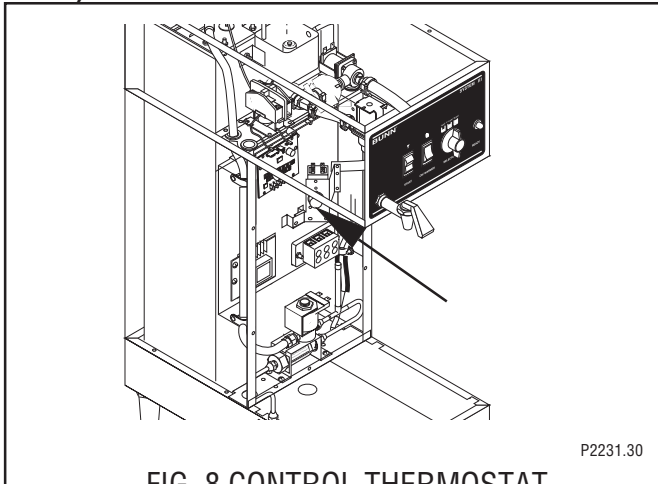
FIG. 8 CONTROL THERMOSTAT
