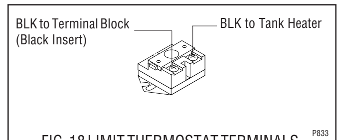
FIG. 18 LIMIT THERMOSTAT TERMINALS
