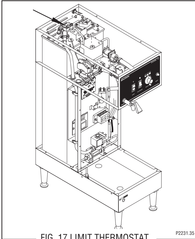
FIG. 17 LIMIT THERMOSTAT
