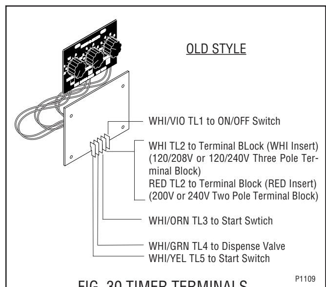
FIG. 30 TIMER TERMINALS
