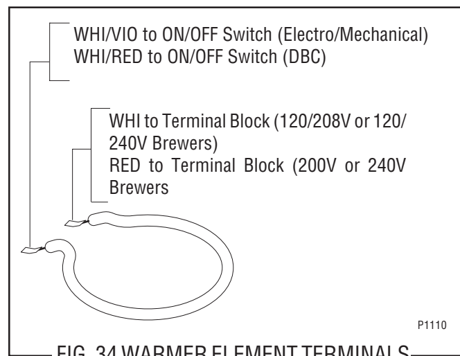
FIG. 34 WARMER ELEMENT TERMINALS
