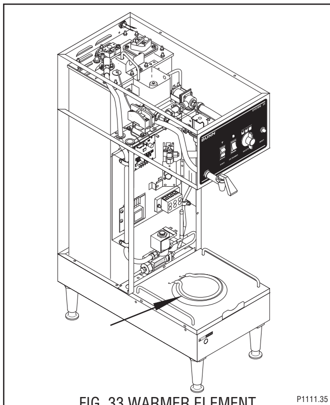
FIG. 33 WARMER ELEMENT
