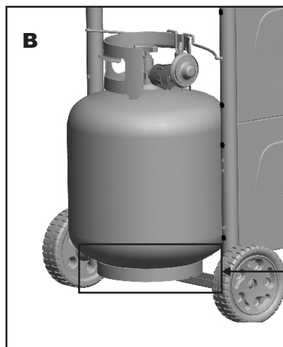
Correctly Installed LP cylinder.
