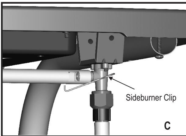
Correctly assembled valve in burner tube and venturi clips
