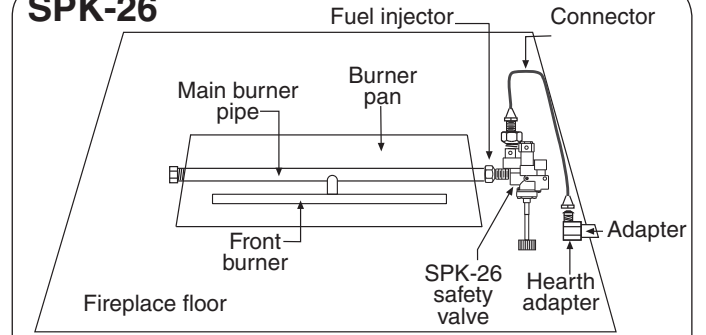
SPK-26 Valve
