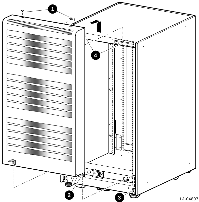
Figure 2-4 Removing and Replacing the Rear Lift-Off Door
