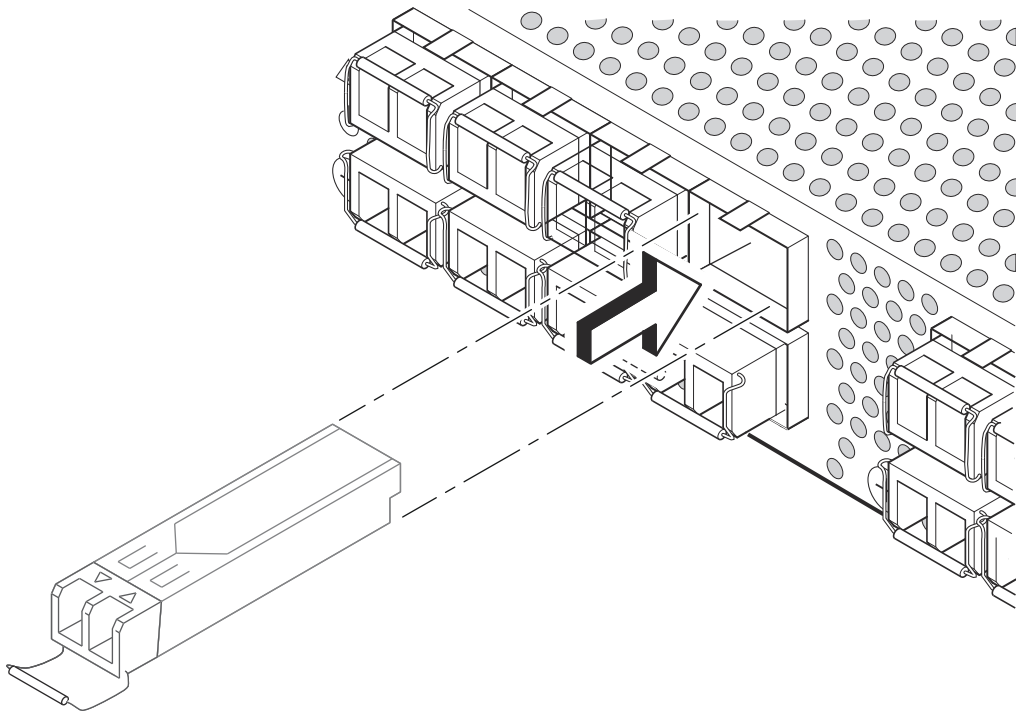
FIGURE 1 Installing an SFP+ transceiver in the upper row of port slots
