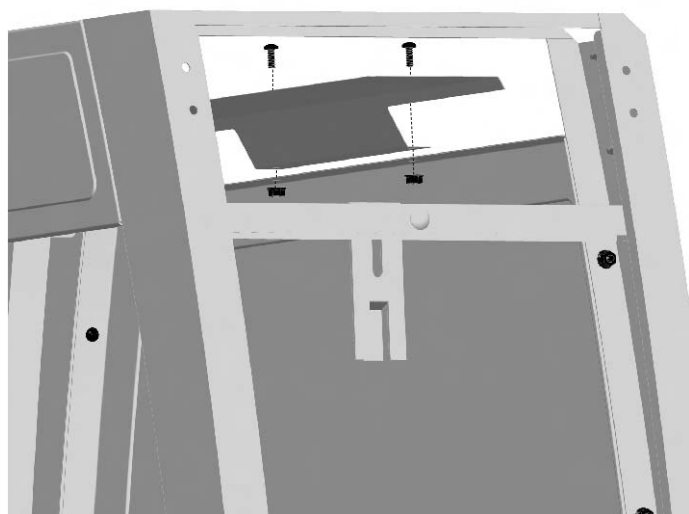
Back view of heat shield
