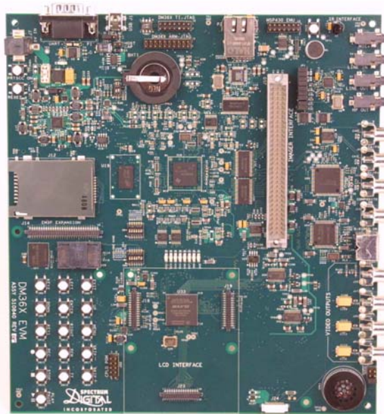
Figure 1-2, DM368 EVM Without DM368 UIM
