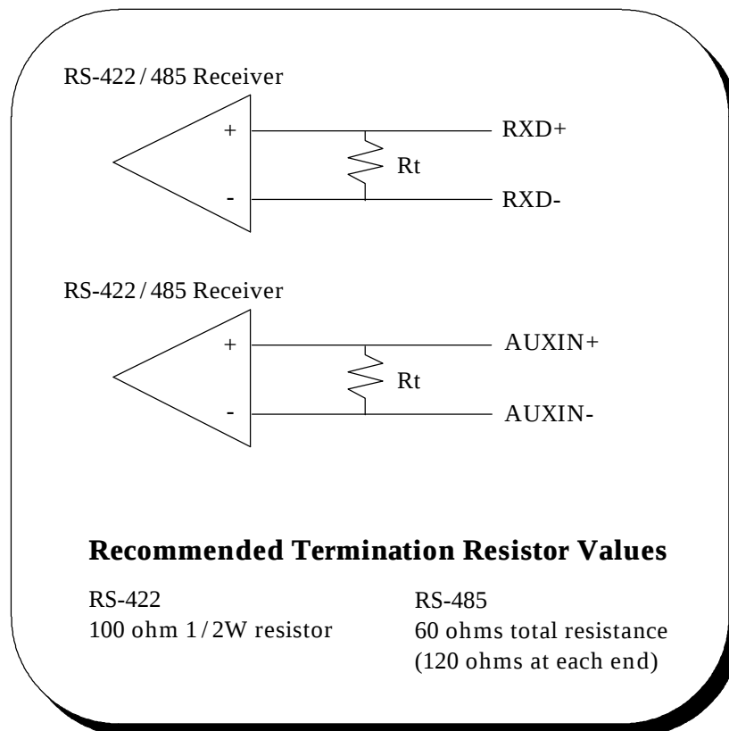
Figure 12. RS-422/485 Termination
