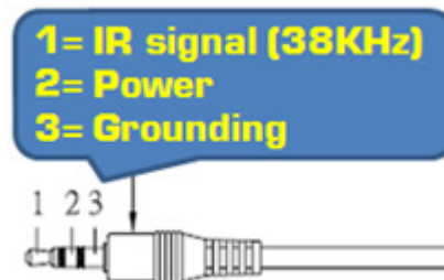
IR Receiver
