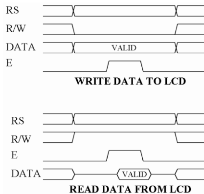
Figure 52 - Serial LCD Graphical Display
