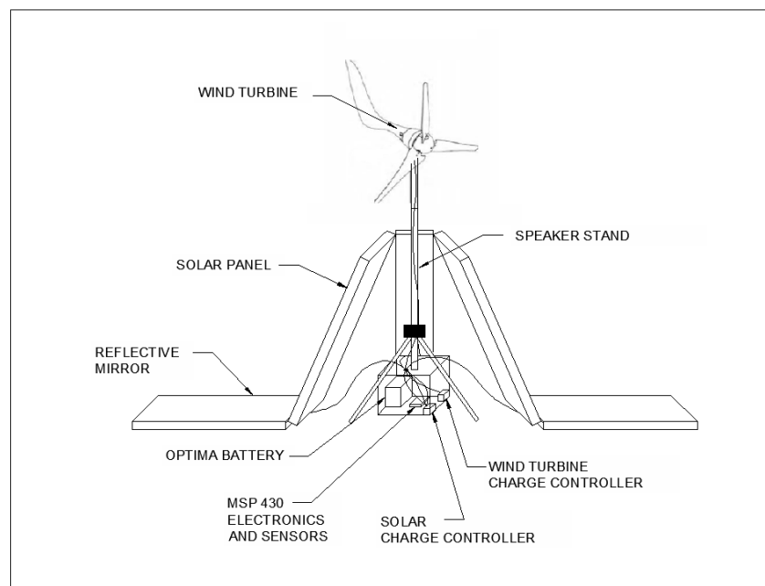
Figure 64 - Overall Concept Design
