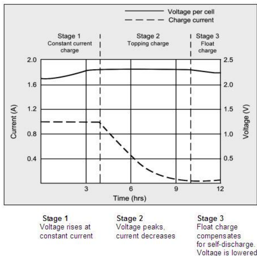
Figure 7 – Lead Acid Battery Charging Stages
