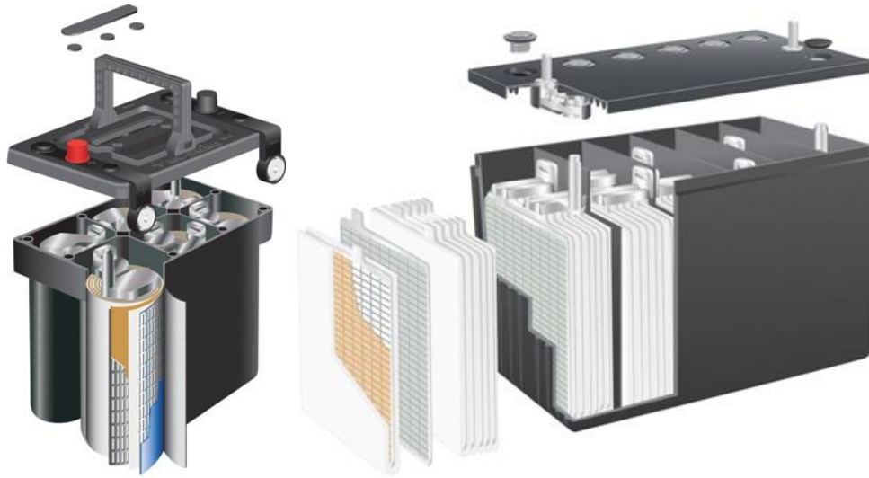
Figure 37 - Spiral Cell vs. Rectangular Cell AGM Battery
