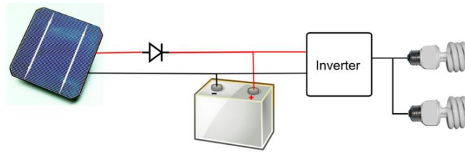
Figure 68 - Connection between PV array and Battery
