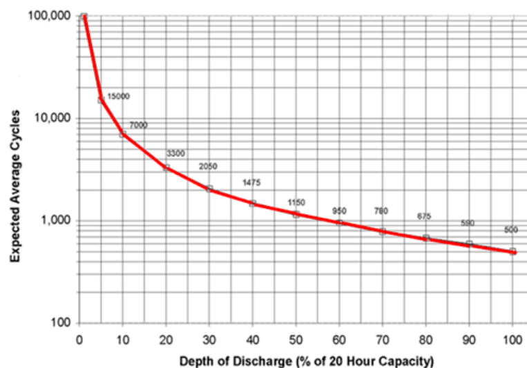
Figure 36 - Cycle Life vs. Depth of Discharge
