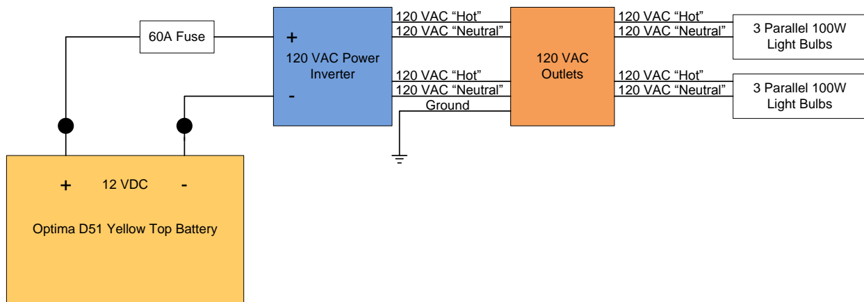
Figure 71 - Schematic for Testing Power Storage System
