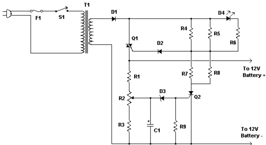
Figure 6 – Lead Acid Battery Charger Circuit
