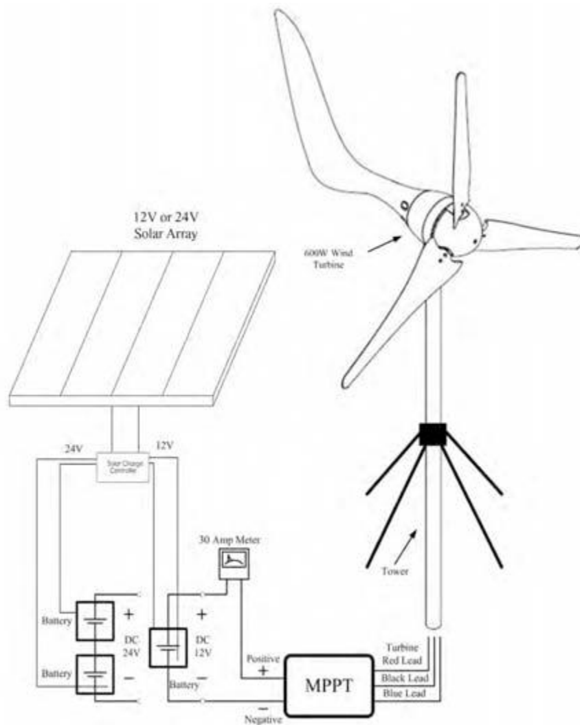
Figure 45 – Solar/Wind Charging Diagram
