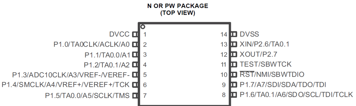
Figure 54 - MSP430G2231 Diagram
