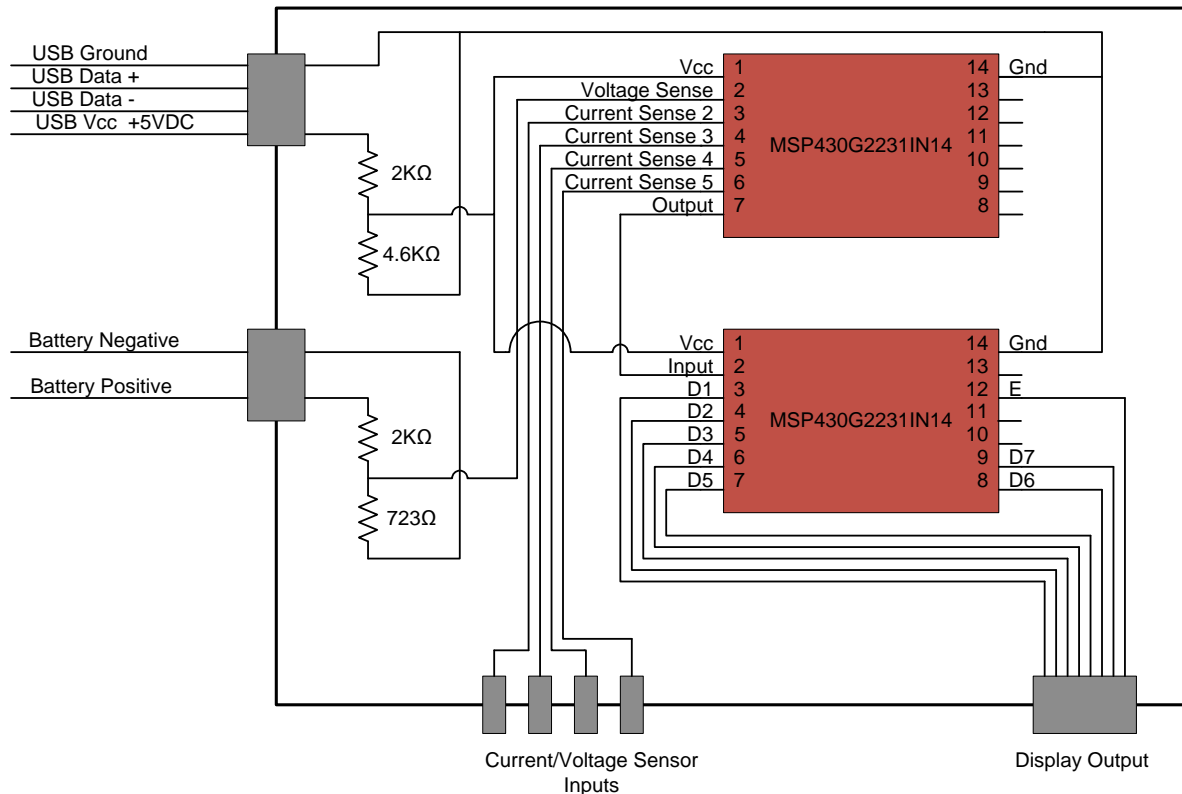
Figure 56 - Planned Schematic of Microcontrollers on PCB
