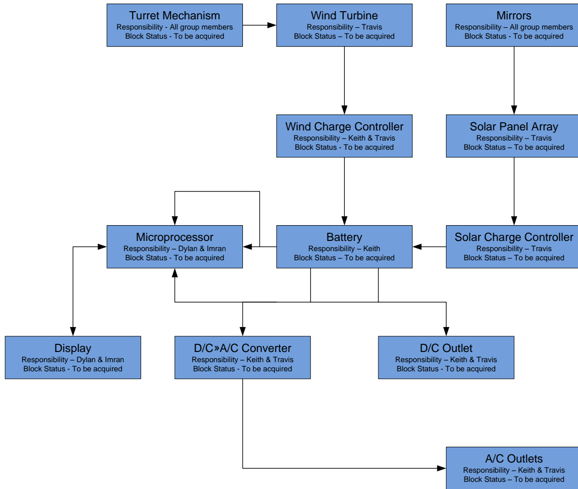
Figure 1 - Block Diagram of Overall System Layout
