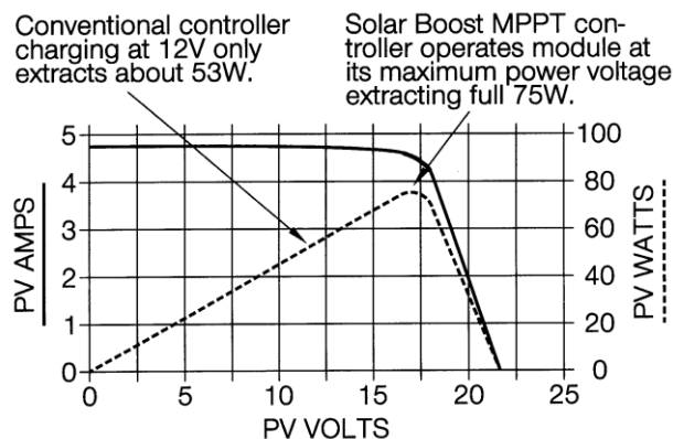
Figure 4 - I-V and P-V Curve of a Typical 75W PV Panel
