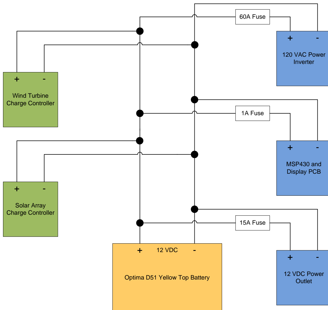
Figure 39 - Schematic Diagram for 12 VDC Supplied by Optima D51 Battery
