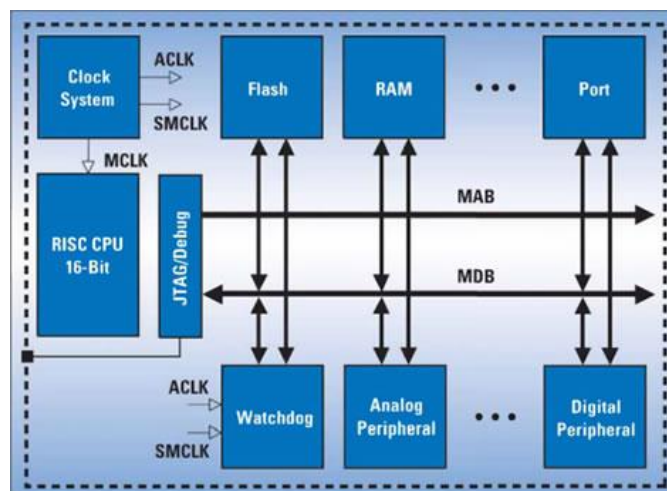
Figure 32 - MSP430 Architecture
