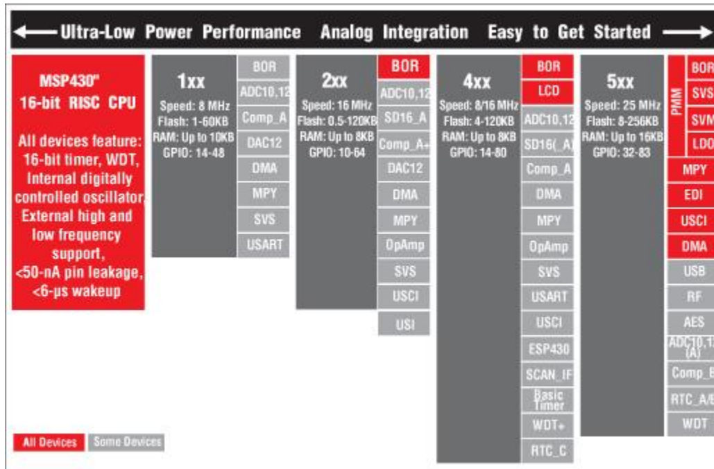
Figure 55 – MSP430 Chart
