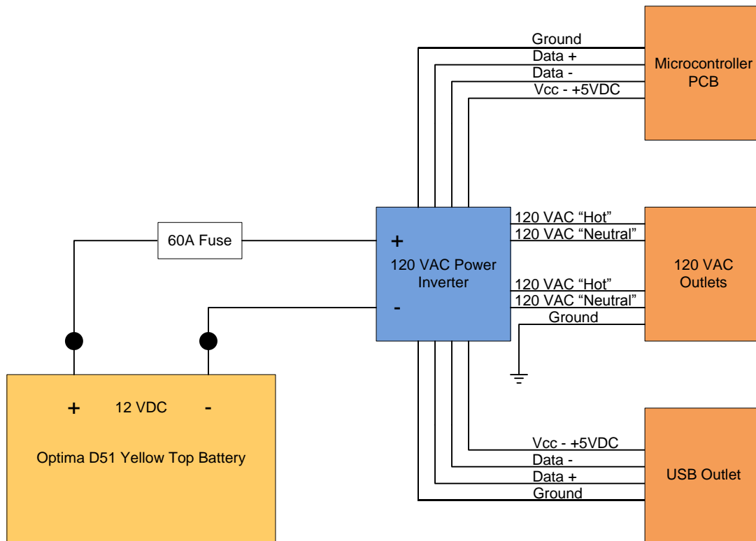
Figure 59 - Schematic Diagram of Wiring from Power Inverter to Outlets
