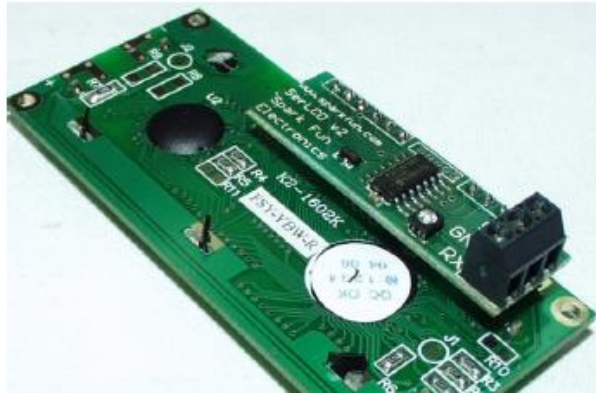
Figure 29 - Serial Connection on LCD
