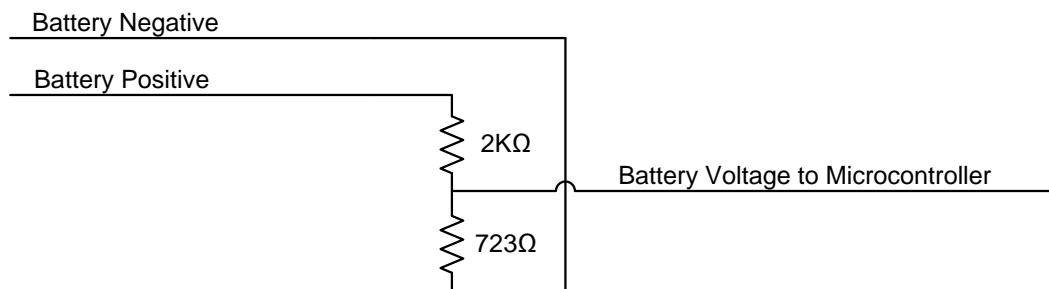
Figure 57 - Voltage Divider to Feed Battery Voltage to Microcontroller
