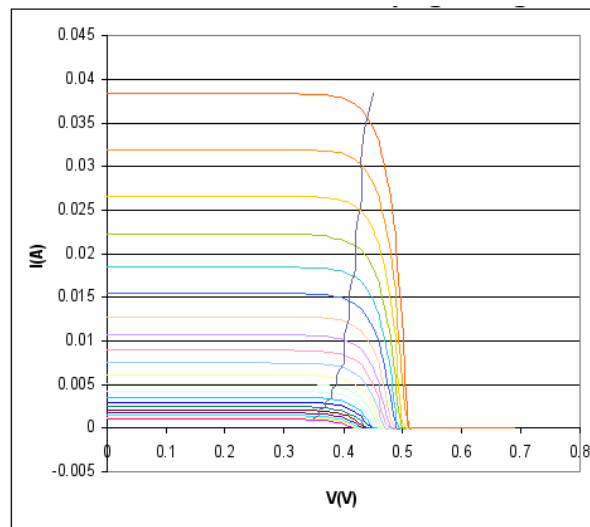
Figure 5 - I-V Curve of a PV Panel at Various Sunlight Levels
