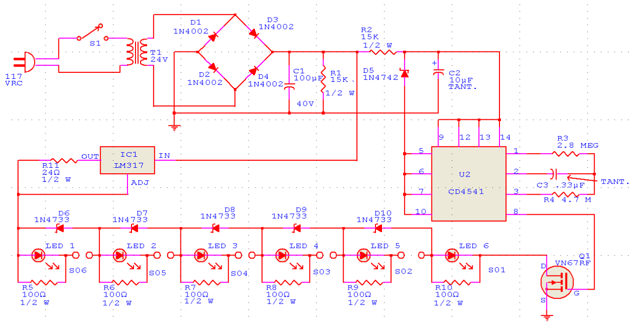
Figure 8 – Nickel-Metal Hydride Battery Charger Circuit
