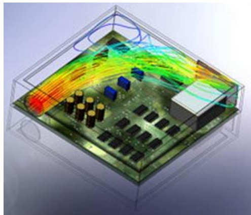
Figure 50 - Airflow Pattern to dissipate heat on board and display
