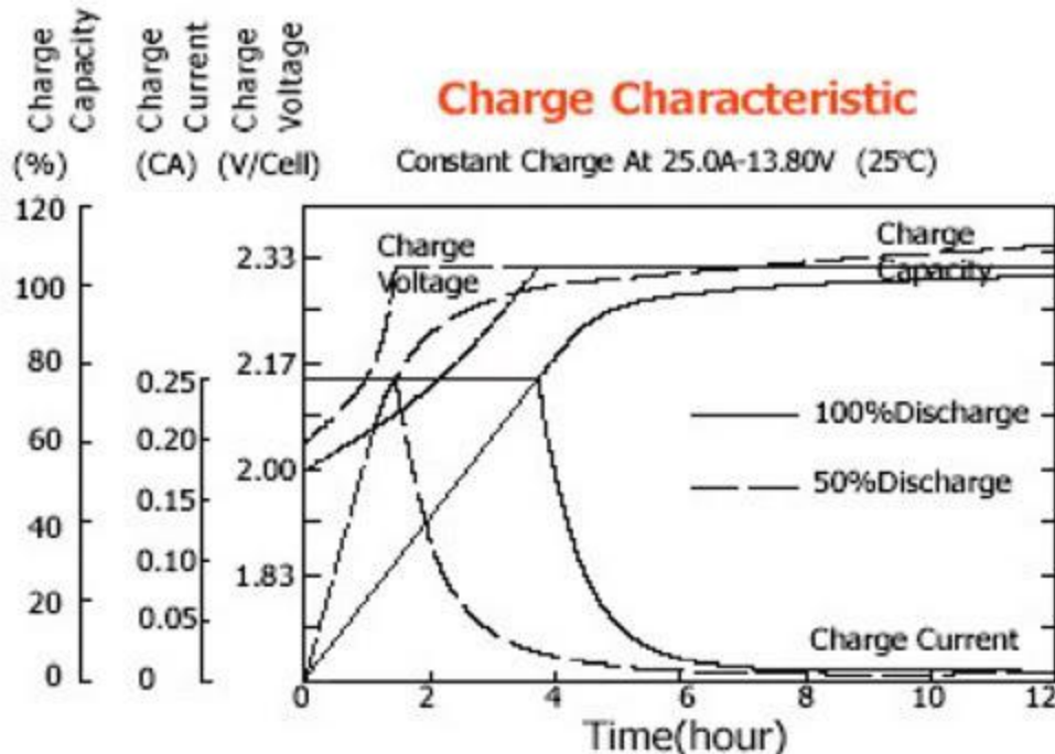
Figure 12 - Charging Stages
