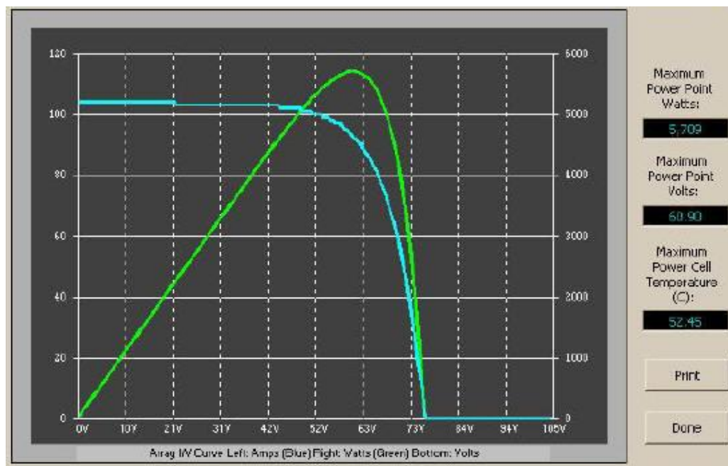
Figure 14 - MPPT Benefit Graph
