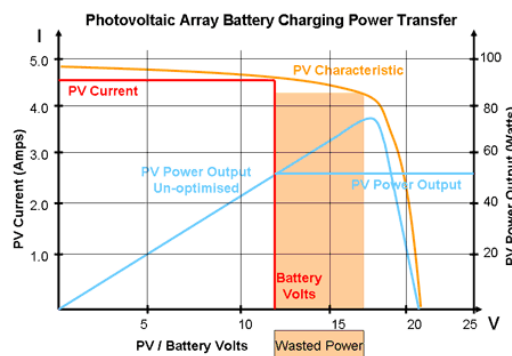
Figure 13 - MPPT Characteristic Graph
