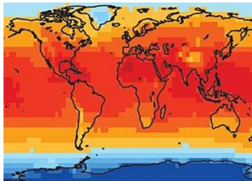
Figure 20 - Global Sun Exposure Map
