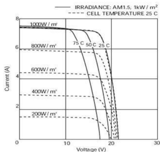
Figure 23 - Current vs. Voltage at Different Temperatures
