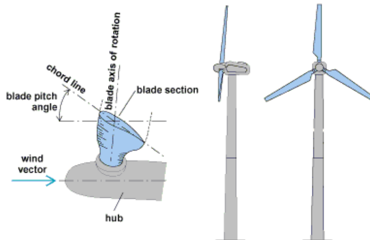
Figure 17 - Horizontal Axis Wind Turbine
