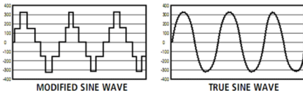
Figure 15 - Modified Sine wave inverter signal vs. pure sine wave inverter signal
