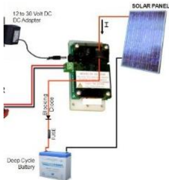
Figure 49 - Current Sensor with DC lines going to battery as well as data lines going to MSP430
