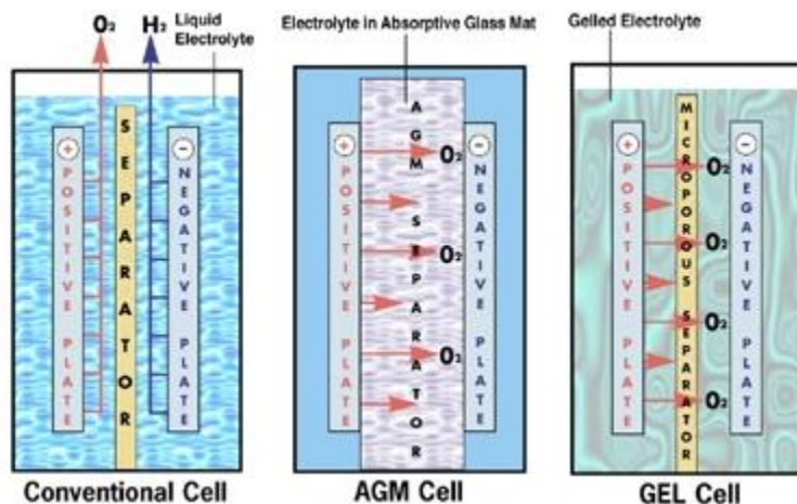
Figure 3 - Comparison between the Construction of Wet Cell, AGM, and Gel Cell Lead Acid Batteries
