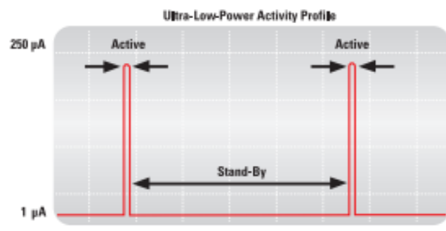
Figure 53 – MSP430 Mpower Consumption
