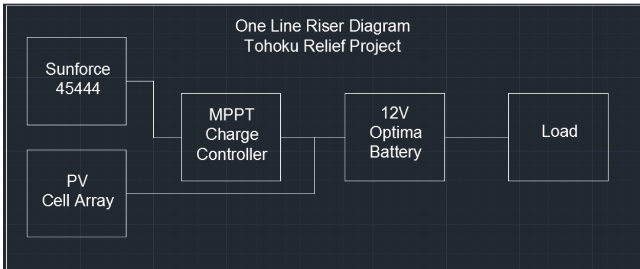
Figure 43 – One Line Diagram
