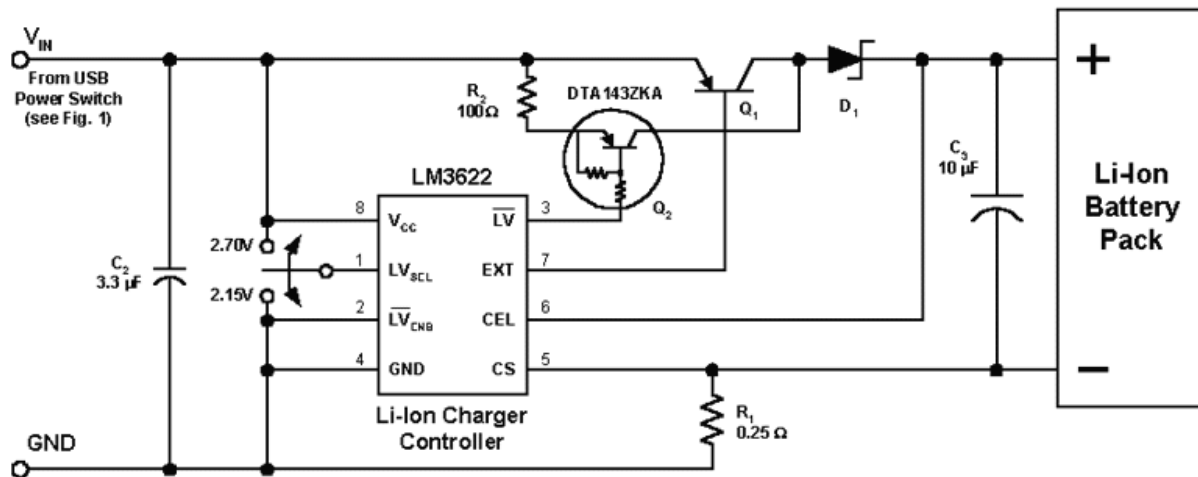
Figure 10 - Lithium Ion Battery Charging Circuit
