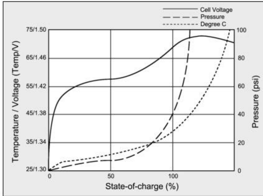
Figure 9 - Charging Characteristics of a Nickel-Metal Hydride Battery
