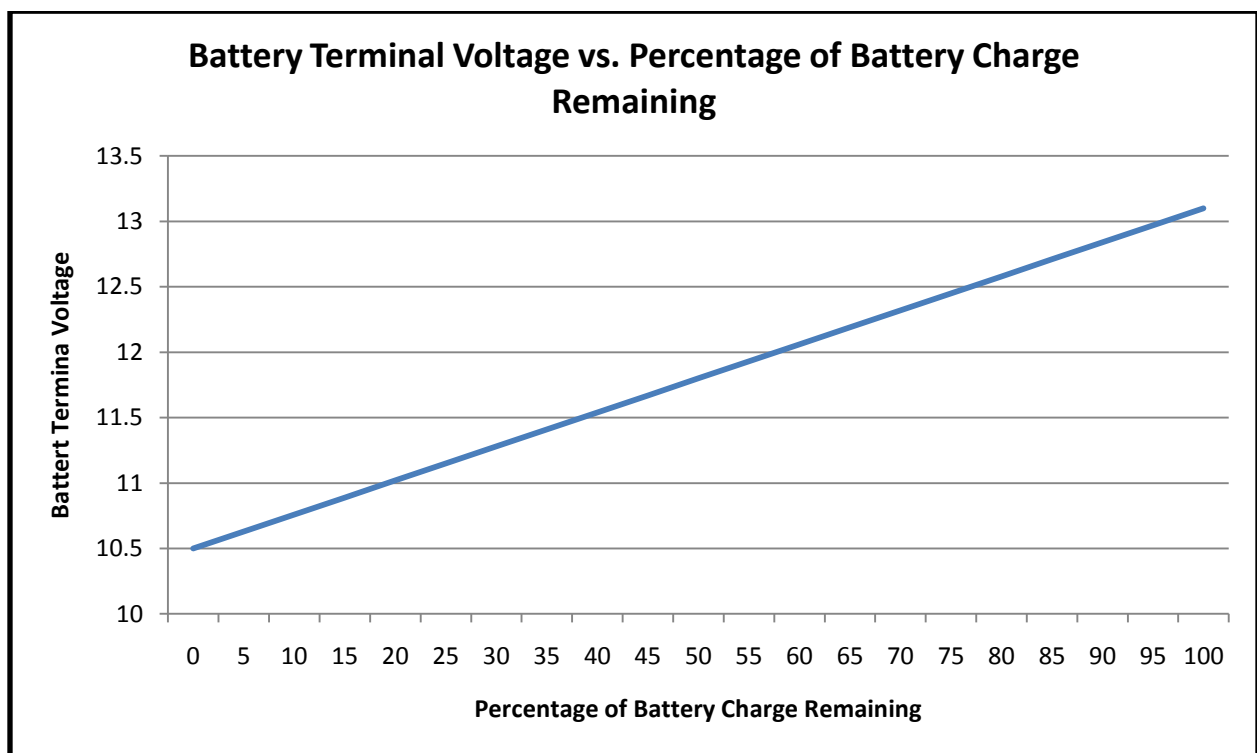
Figure 25 - Battery Terminal Voltage vs. Percentage of Battery Charge Remaining
