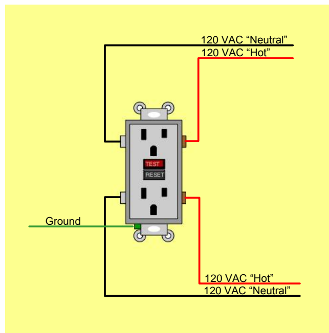
Figure 60 - Wiring Diagram for GFCI Outlet
