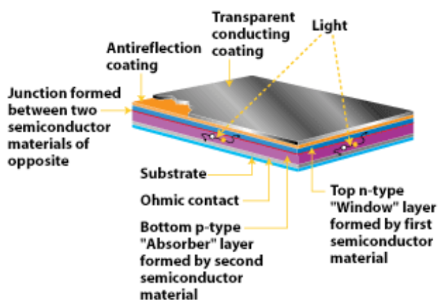
Figure 24 - Thin Film Array Panel Layers
