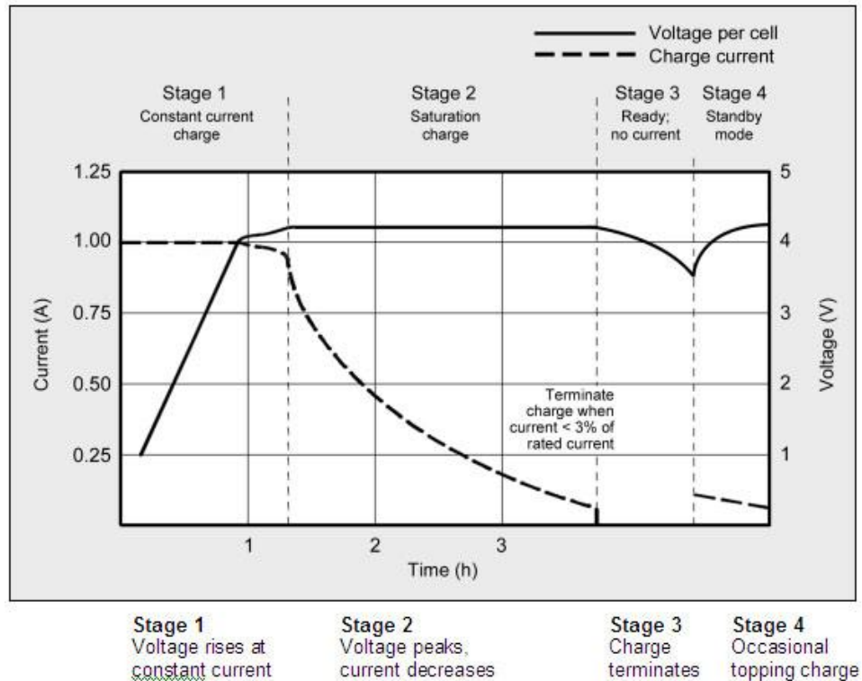
Figure 11 – Charging States of Lithium Ion Battery
