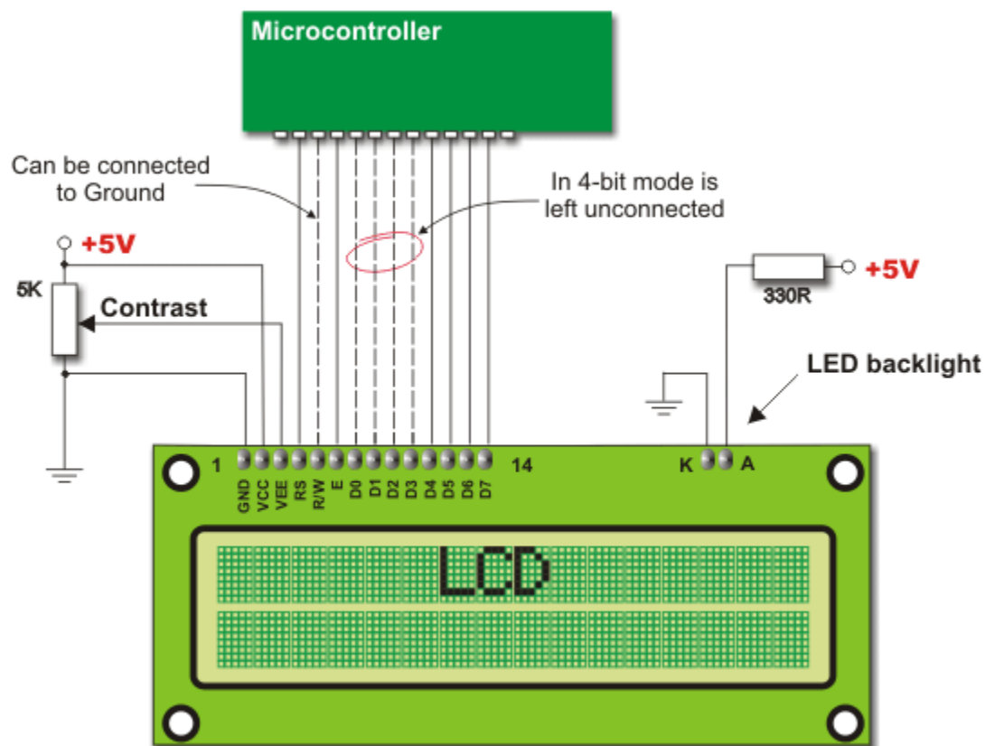
Figure 30 - LCD/Microcontroller Interconnection
