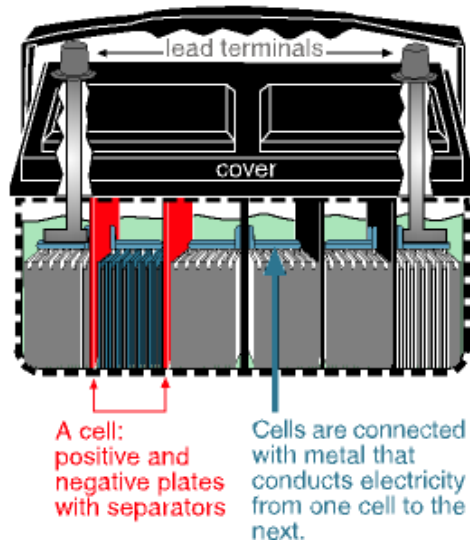
Figure 2 - Typical Construction of a Lead Acid Battery
