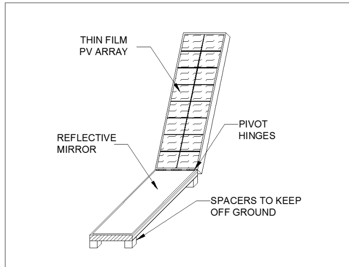
Figure 47 - PV Array
