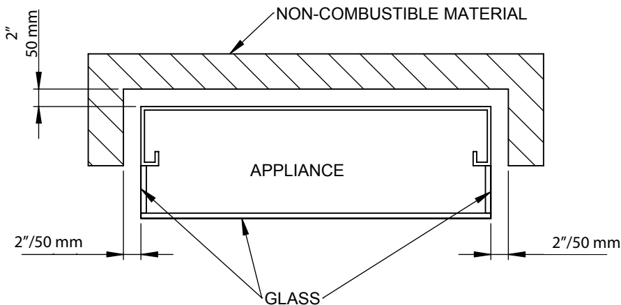
Figure 10 Plan View
