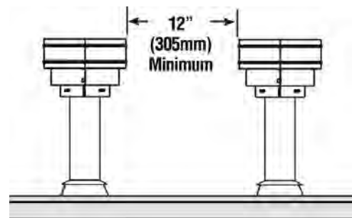
Figure 25. Multiple Termination Clearance
