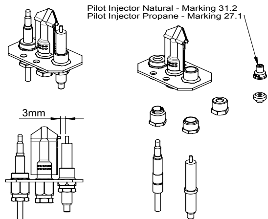
Figure 66. Pilot Burner Detail
