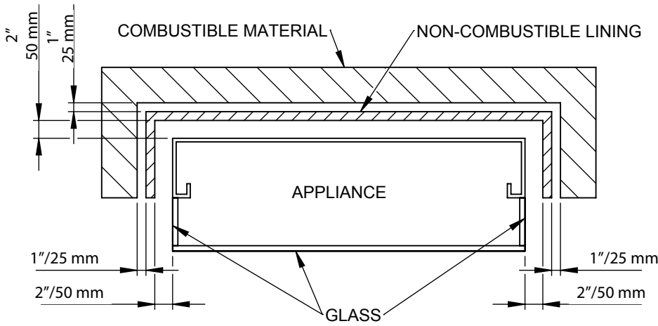
Figure 8 Plan View
