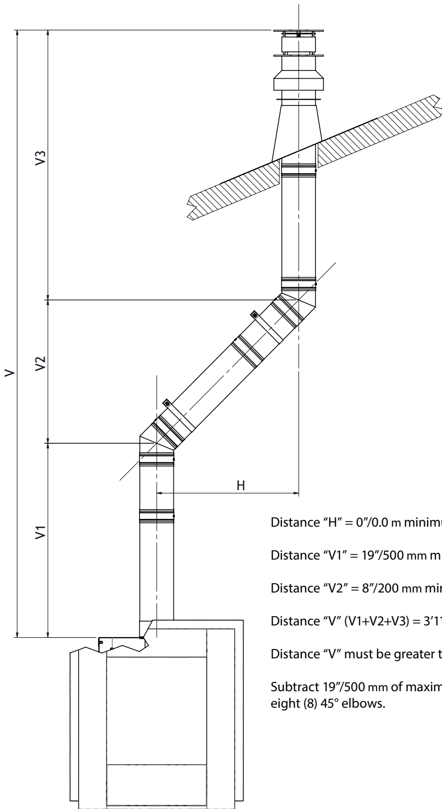
Figure 24. Vertical Terminations with 45° elbows
