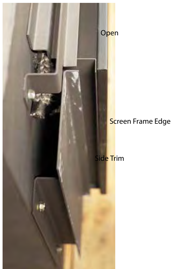
Figure 65 Top View with Screen Attached
