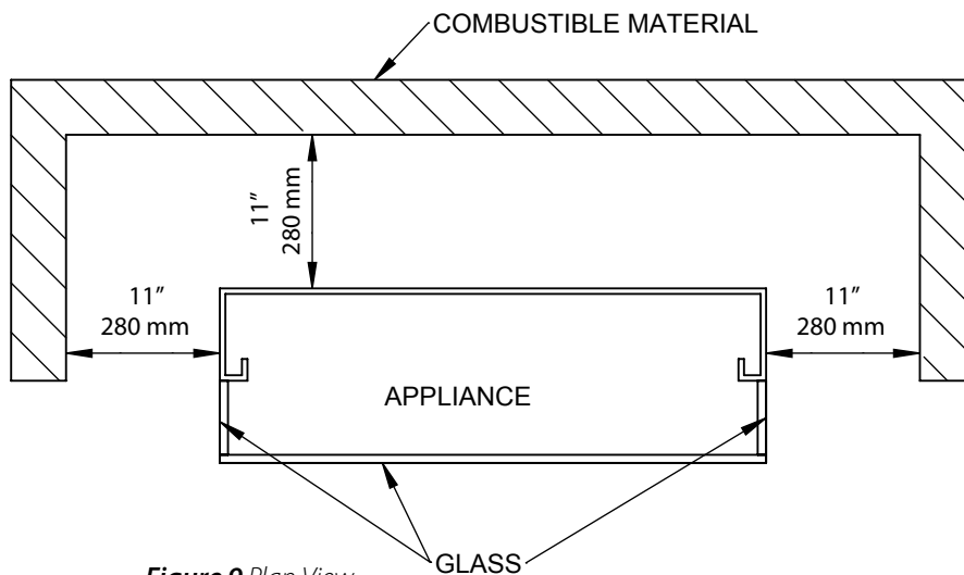
Figure 9 Plan View
