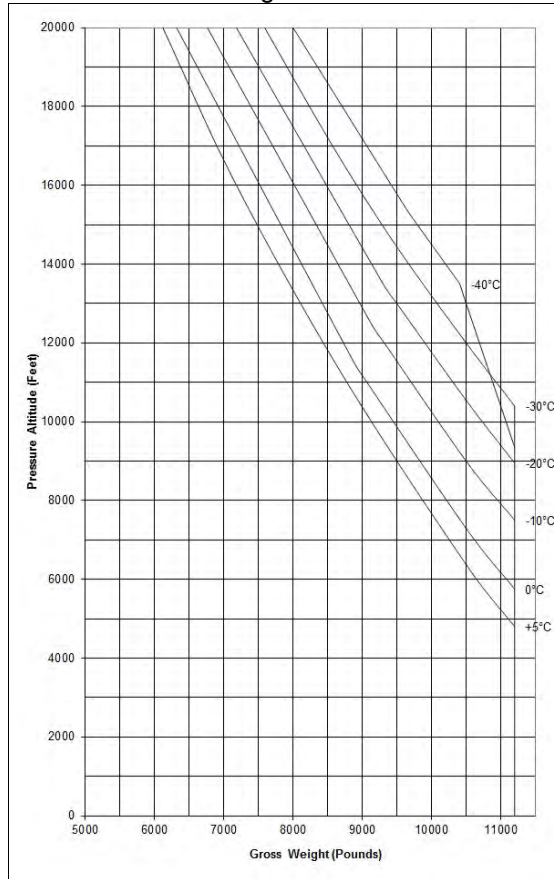
Figure 4-6 – Hover Ceiling (without Particle Separator) (Sheet 4 of 8)
