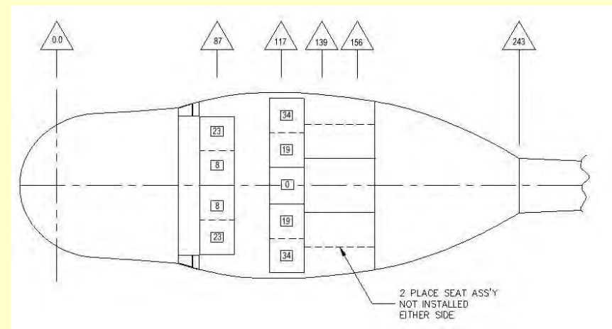
Figure 1-2 – Nine-place passenger loading configuration 2
