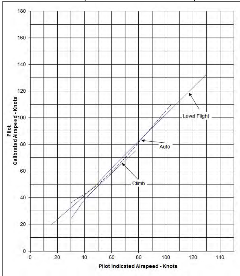
Figure 4-10 – Pilot Airspeed System Calibration
