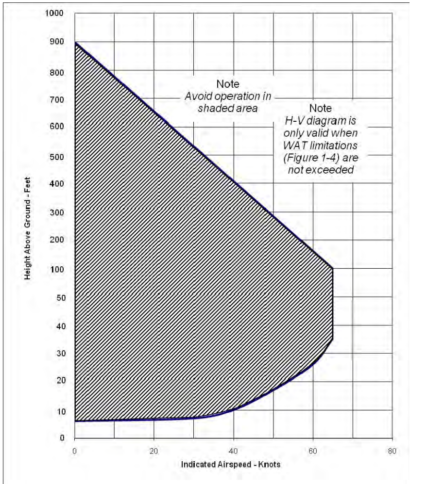
Figure 4-14 – Height Velocity Chart
