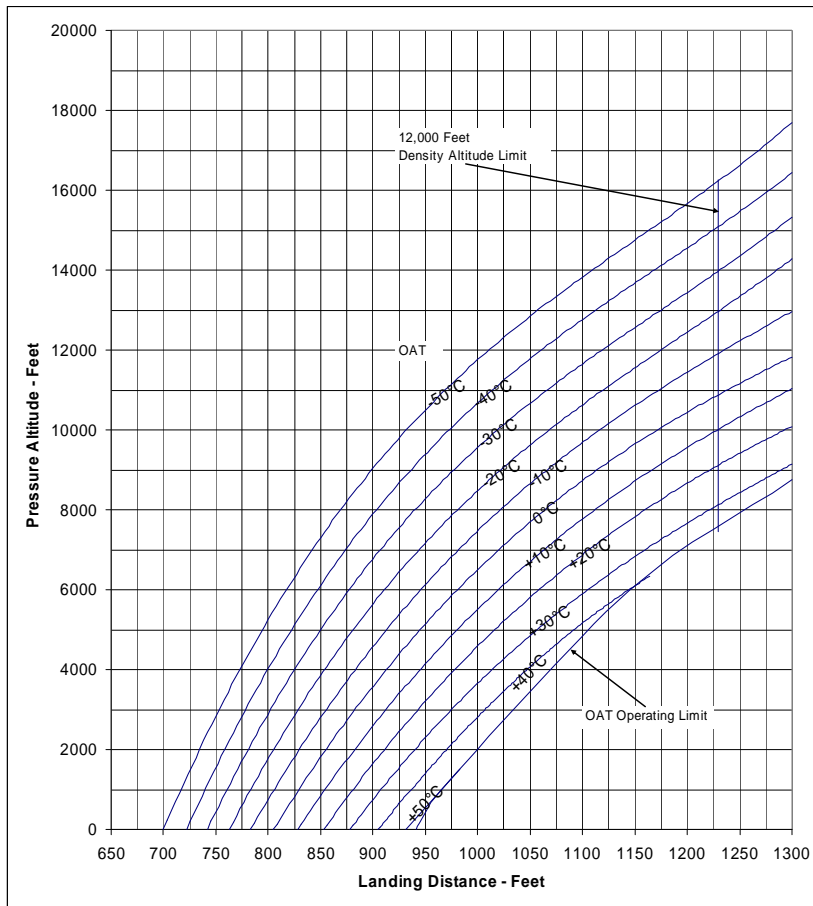
Figure 4-9 – Landing Distance (Sheet 3 of 6)
