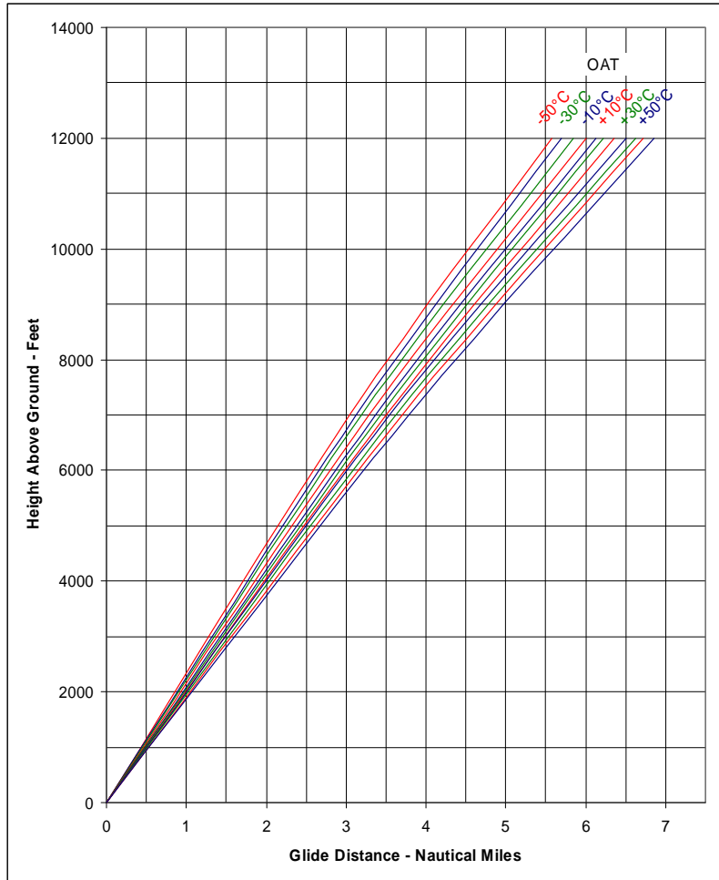
Figure 4-12 – Glide Distance
