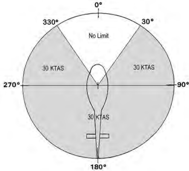
Figure 4-5 – Operation vs Allowable Wind 10,500 Lbs and Below
