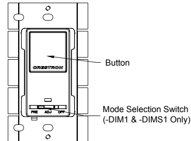
Buttons of CLW-DIM1, -DIMS1, and -SLVD1
