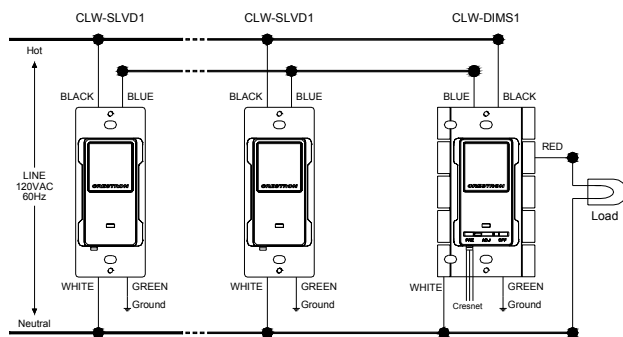
Wiring Diagram of CLW-DIMS1 with multiple CLW-SLVD1s
