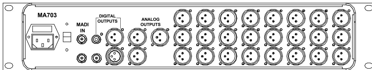
Figure 2-3 MA703 Rear Panel
