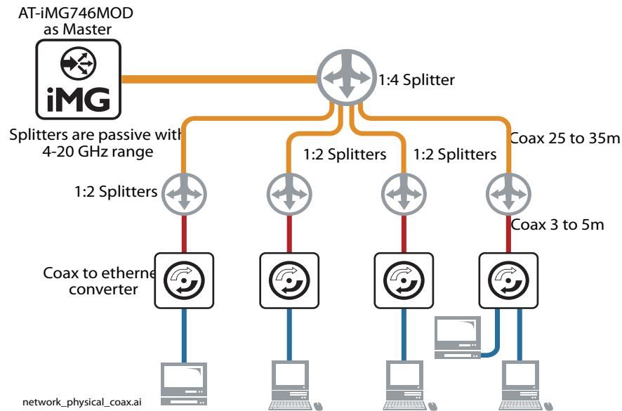
Figure 24. Coax Network Configuration
