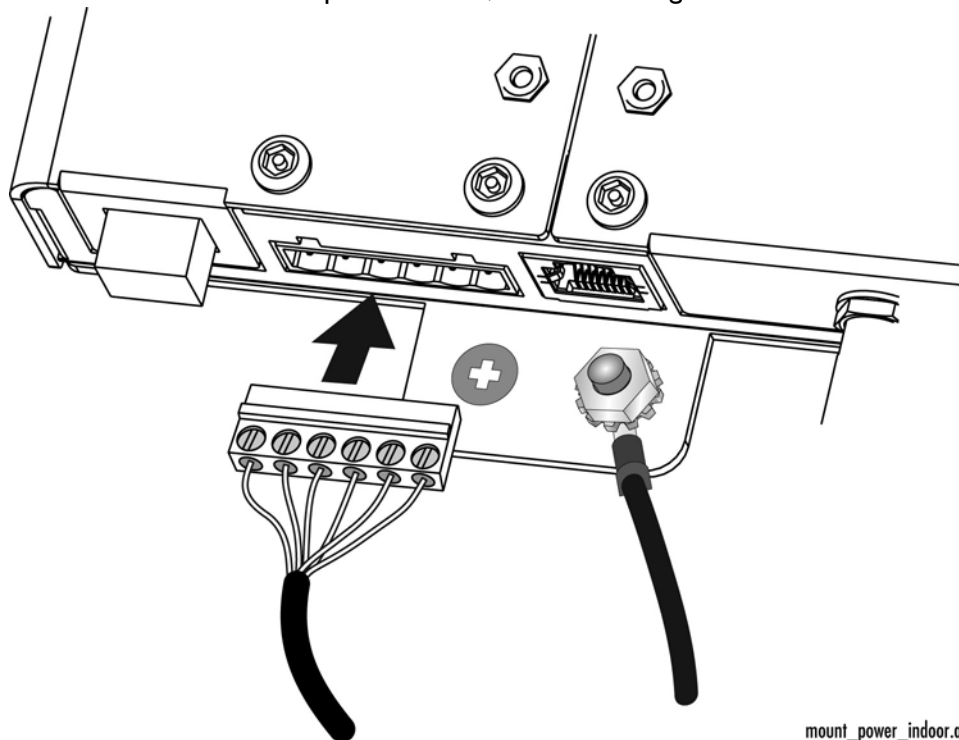
Figure 22. Plugging in the DC Terminal Block
