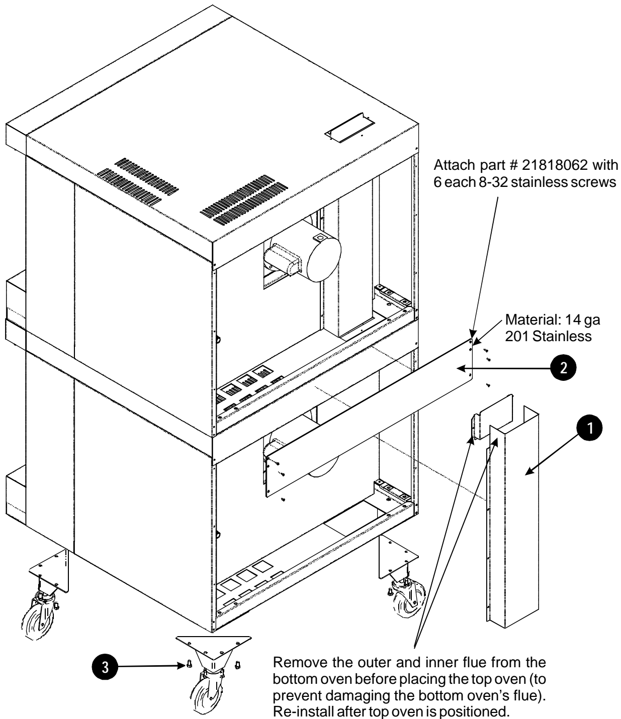
Figure 3 STACKING INSTRUCTIONS FOR: BCO-G & GDCO-G CONVECTION OVENS
