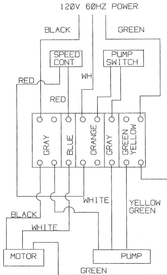
QC36DVS 36" VARIABLE SPEED WIRING DIAGRAM
