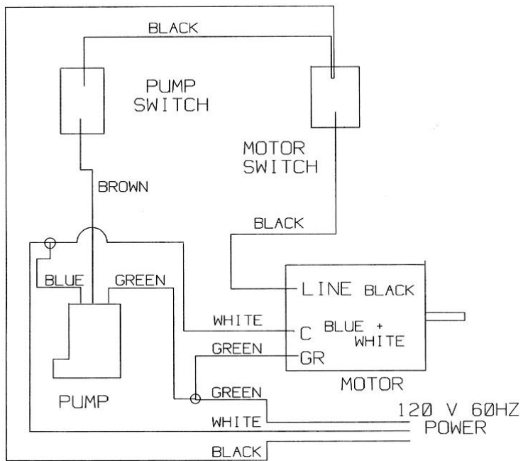
QC36D1 - 1/2 HP 1 SPEED WIRING DIAGRAM
