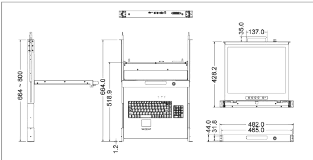
Figure 1-3. Unicorn 19 Dimension
