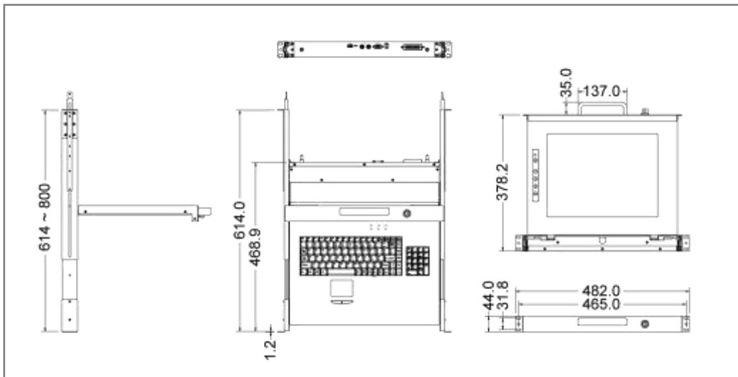
Figure 1-1. Unicorn 15 Dimension
