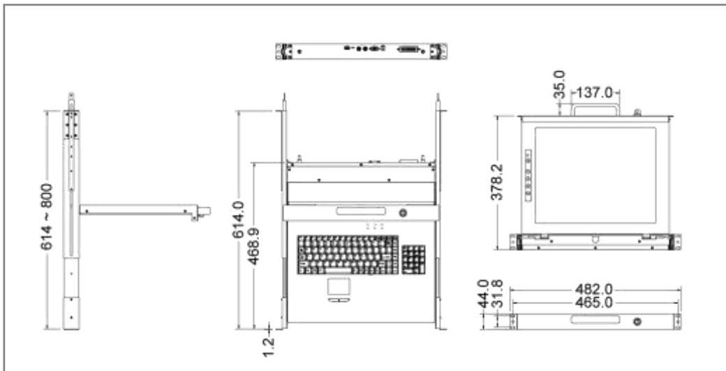
Figure 1-2. Unicorn 17 Dimension
