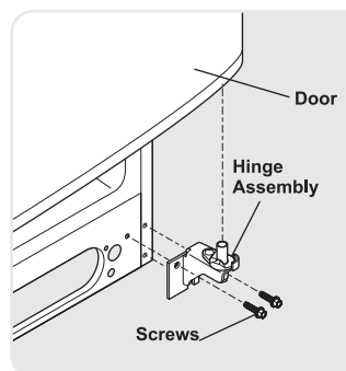
Non-Adjusting Hinge (some models)
