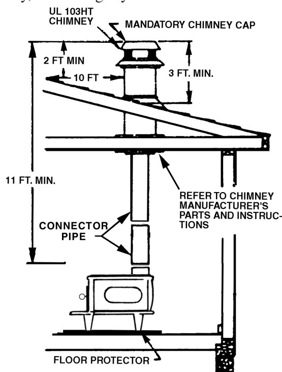
Fig. 5 - Chimney Construction Through Attic Space
