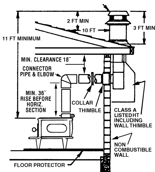
Fig. 7 - Chimney Connection to Firebox Through Masonry Wall
