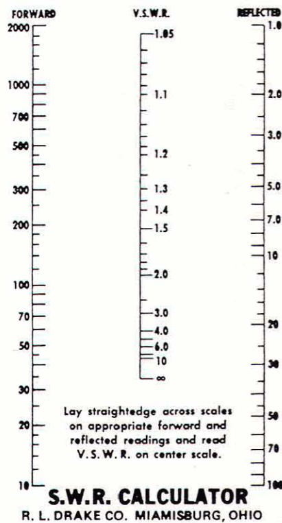
Figure 3-3. SWR Nomograph
