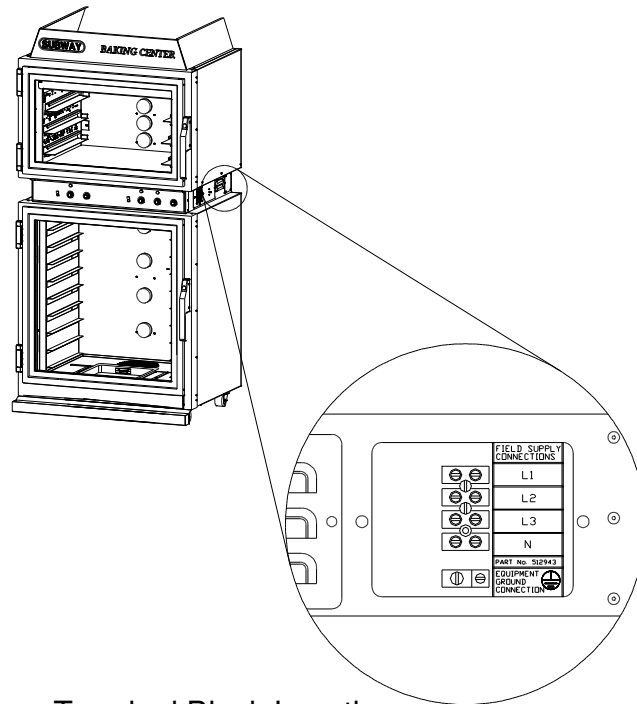
Terminal Block Location
