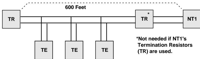
Figure 5. Short Passive Bus Configuration
