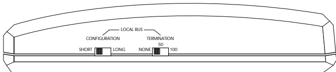
Figure 3. Switch Locations
