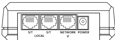
Figure 2. Interface Connectors
