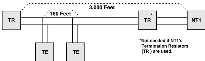
Figure 6. Extended Passive Bus Configuration
