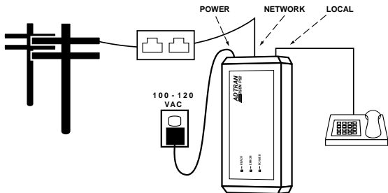
Figure 4. Power Supply Connection
