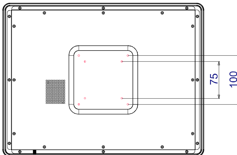
Figure 11 Mounting hole locations
