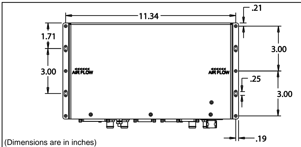
Figure 2 Dimensions for the mounting holes
