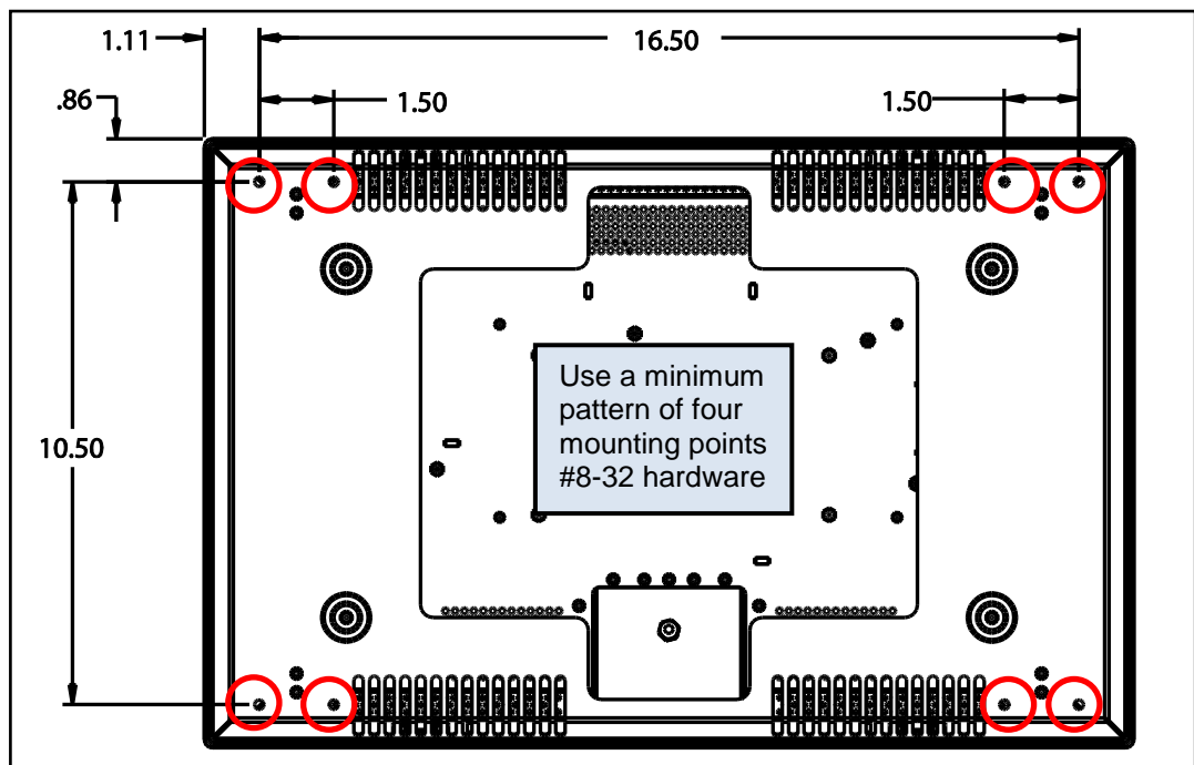
Figure 5 Rear view of the 19" cosmetic back (shown with chassis) for a proud mount
