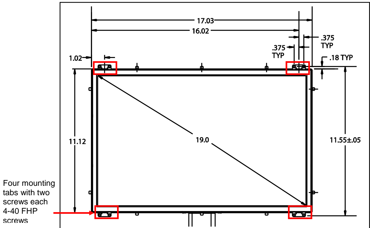
Figure 4 Front view of a 19" flush or semi-proud mount from the front tabs
