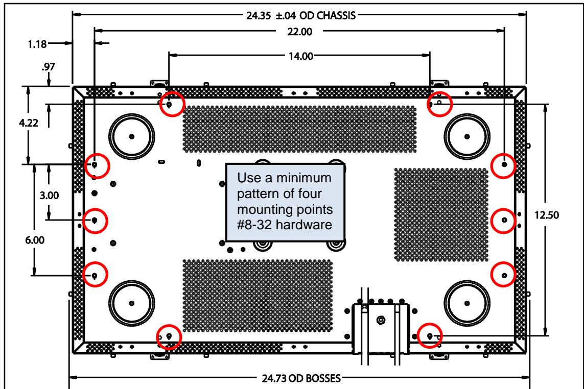
Figure 9 Rear view of a 26" flush mount
