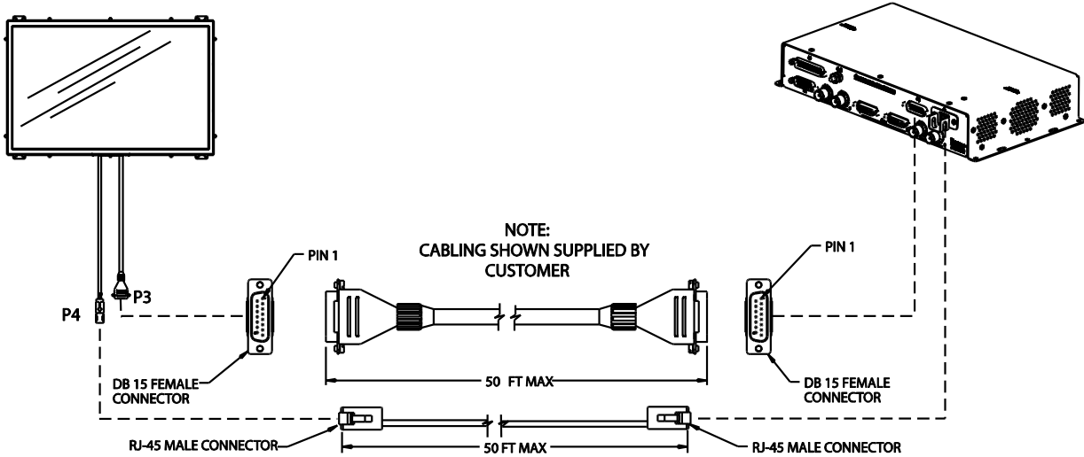
Figure 13 Remote display system connections
