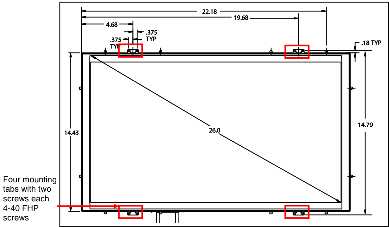
Figure 10 Front view of a 26" flush or semi-proud mount from the front tabs
