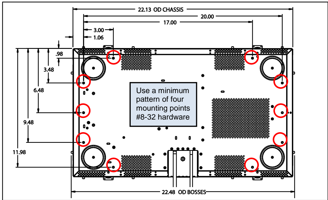
Figure 6 Rear view of a 24" flush mount
