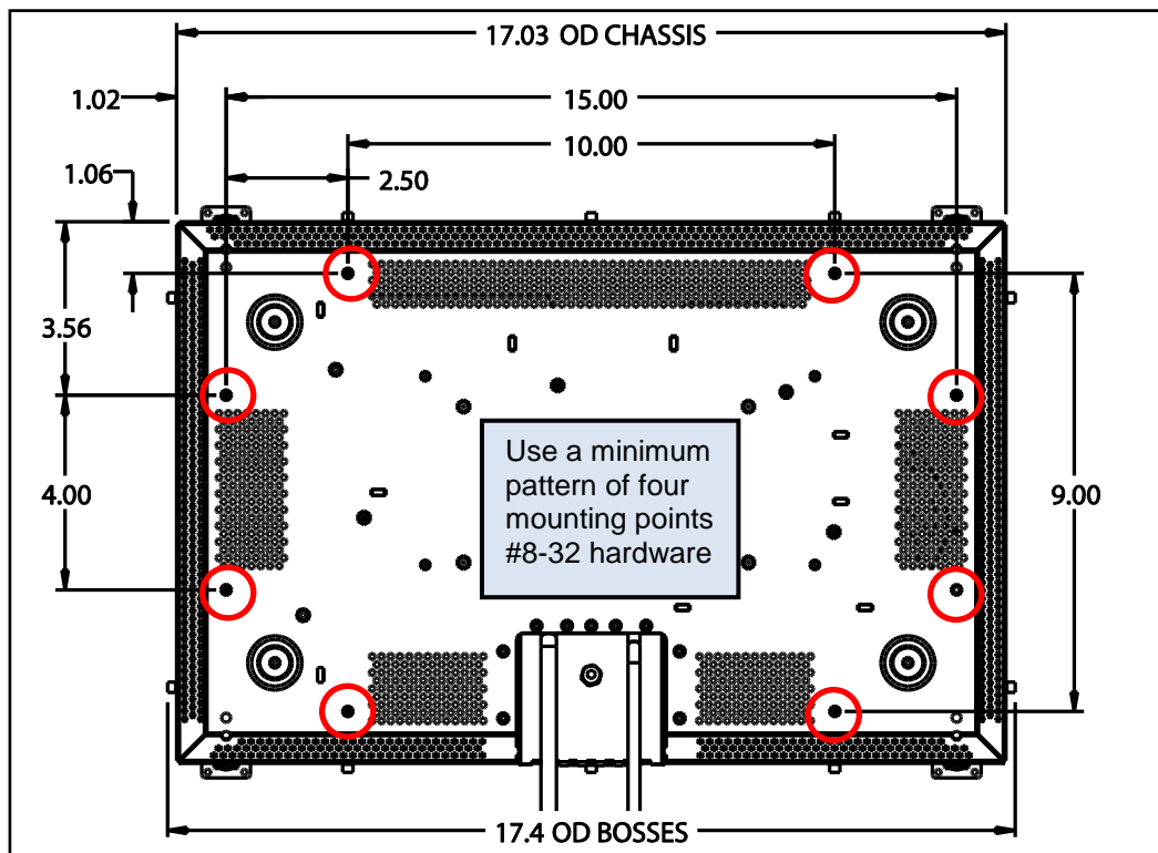
Figure 3 Rear view of a 19" flush mount
