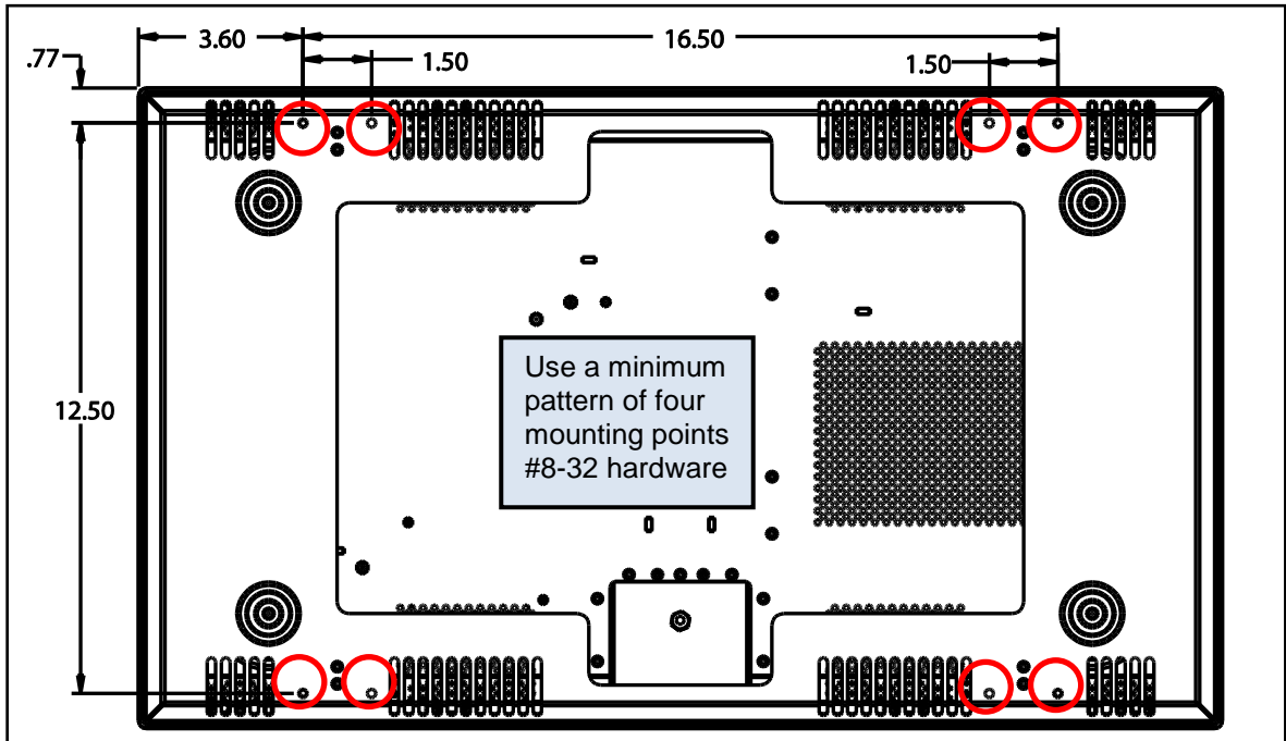
Figure 8 Rear view of the 24" cosmetic back (shown with chassis) for a proud mount
