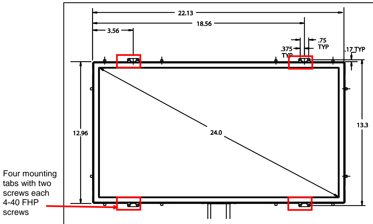
Figure 7 Front view of a 24" flush or semi-proud mount from the front tabs
