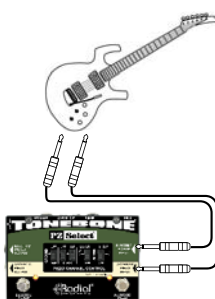
Dual TS Cable: Tip and Ring are routed to separate phone connectors.
