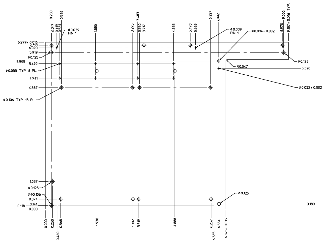
Figure 4-18 PMC Expansion Adapter
