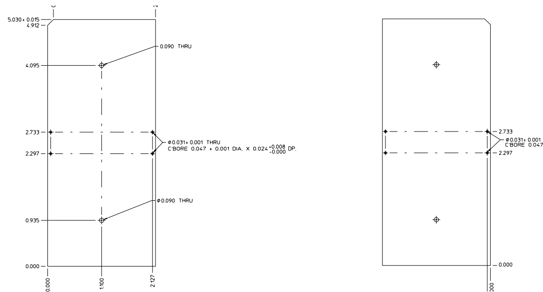
Figure 4-14 Model 744 RAM Card (Continued)
