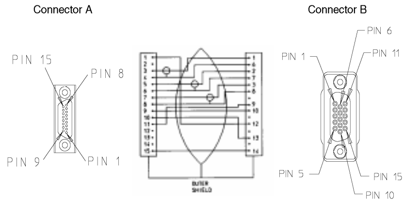
Figure 5-3 HP A4223A Conversion Video Cable Connectors
