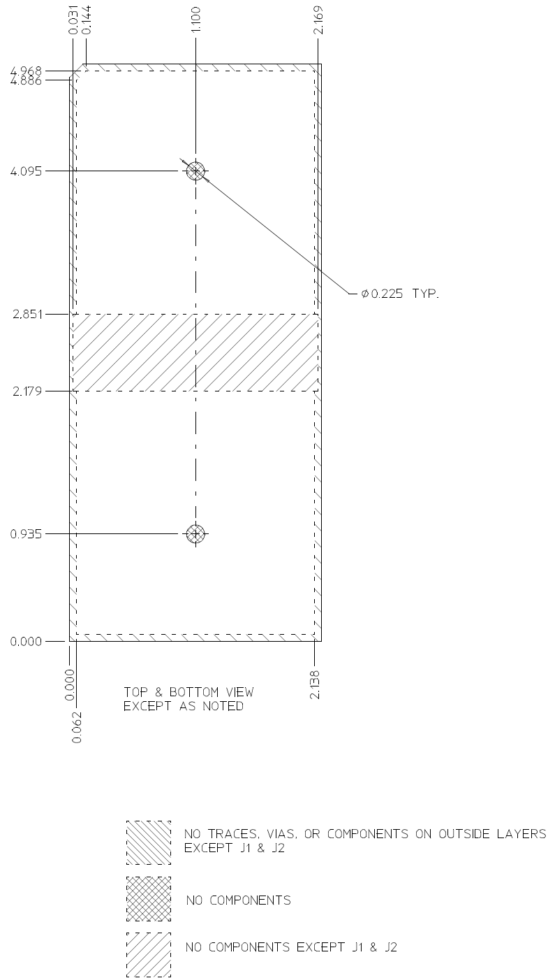
Figure 4-15 Model 744 RAM Card (Continued)
