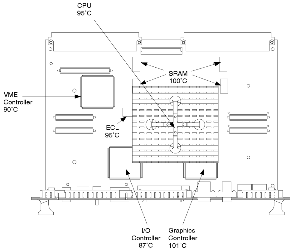
Model 743 Integrated Circuit Case Temperature Limits
