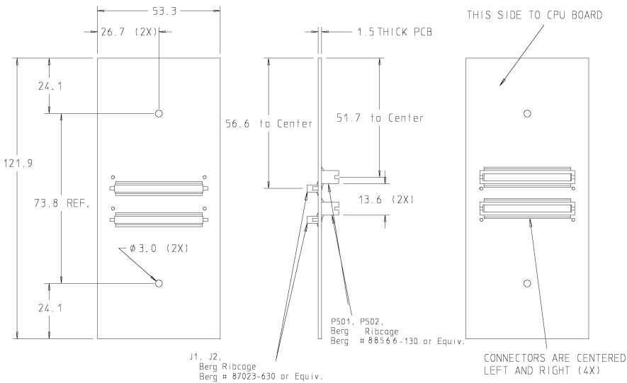
Figure 4-7 Model 743 RAM Card
