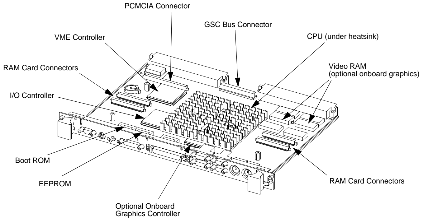
Figure 1-2 Model 743 VME Board Computer Functional Components
