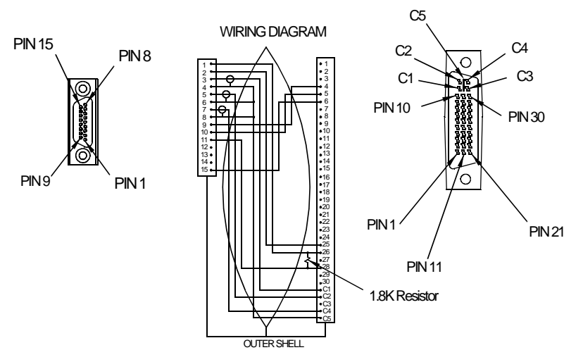
Figure 5-4 HP A4305A Conversion Video Cable Connectors
