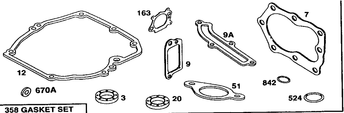
358 GASKET SET
