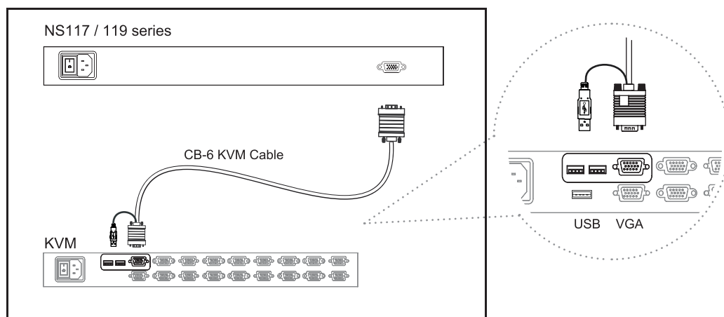
Figure 11. Example of connecting CB-6 2-in-1 USB KVM cable to KVM via USB interface
