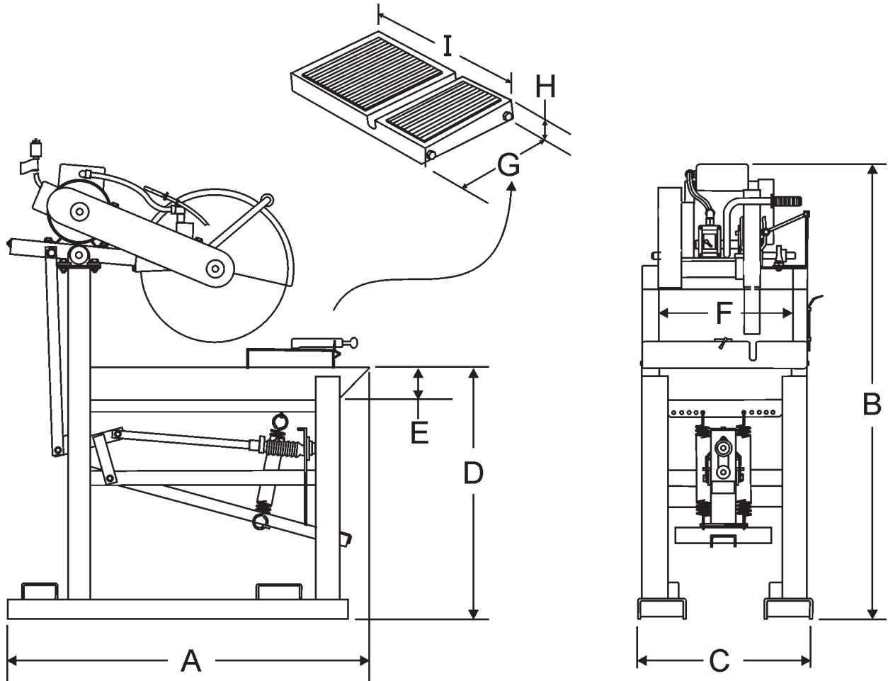
Figure 1. MP2 Dimensions
