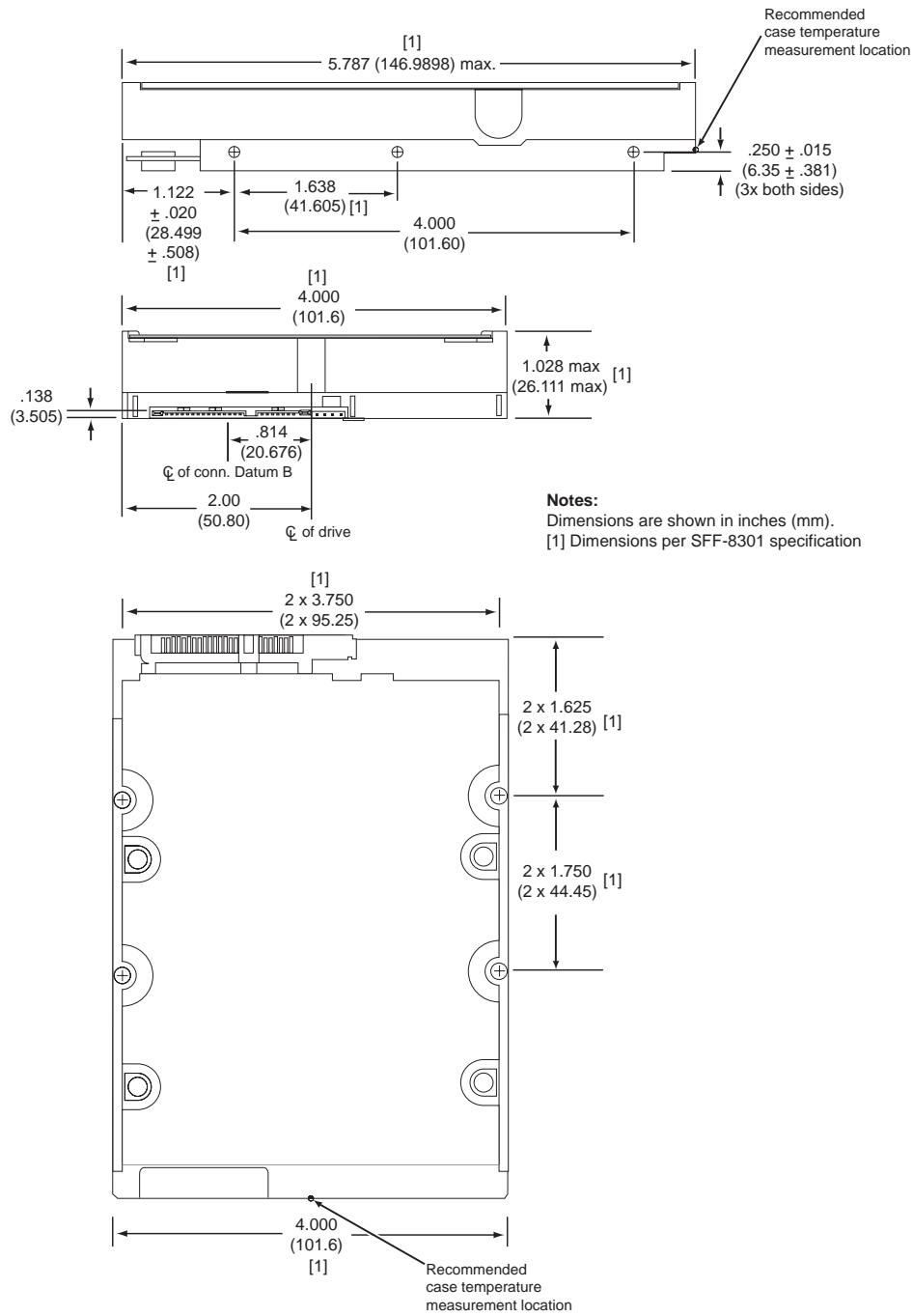
Figure 5. Mounting dimensions
