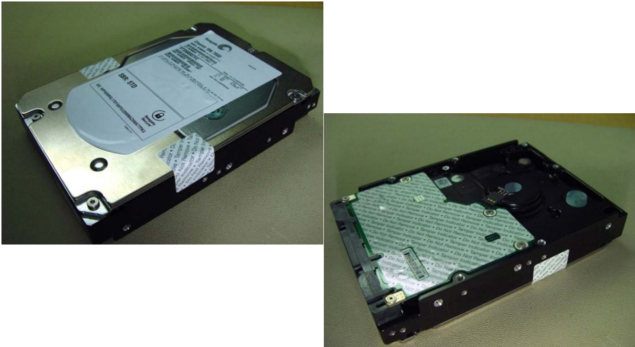
Figure 16. Example of FIPS tamper evidence labels.
