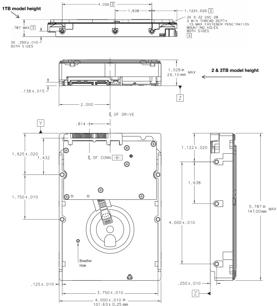
Figure 7 Mounting dimensions
