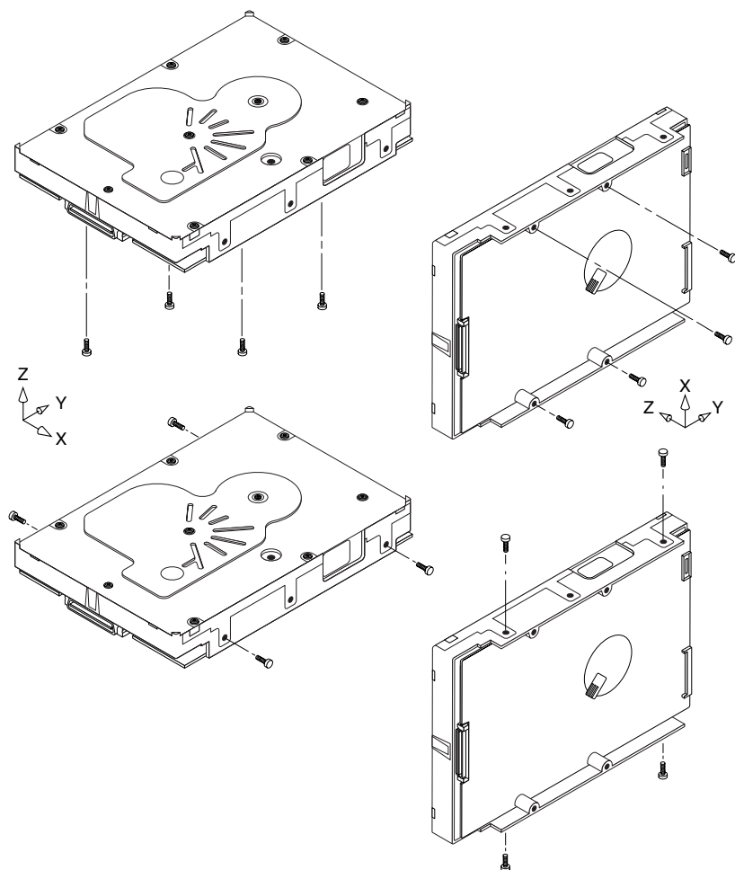
Figure 6. Recommended mounting
